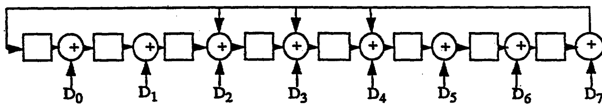
Fig. 2 (Prior Art)
