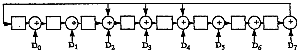
Fig. 2 (Prior Art)
