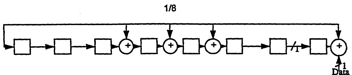
Fig. 1 (Prior Art)
