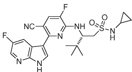
(S)-2-((5-Cyano-3-fluoro-6-((S)-2-((5-fluoro-1H-pyrrolo[2,3-b]pyridin-3-yl)pyridin-2-ylamino)-N-cyclopropyl-3,3-dimethylbutane-1-sulfonamido)-5-fluoro-1H-pyrrolo[2,3-b]pyridin-3-yl)pyridin-2-ylamino)-N-cyclopropyl-3,3-dimethylbutane-1-sulfonamide (28)
