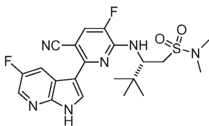
(S)-2-((5-Cyano-3-fluoro-6-((S)-2-((5-fluoro-1H-pyrrolo[2,3-b]pyridin-3-yl)pyridin-2-ylamino)-N,N,3,3-tetramethylbutane-1-sulfonamido)-5-fluoro-1H-pyrrolo[2,3-b]pyridin-3-yl)pyridin-2-ylamino)-N,N,3,3-tetramethylbutane-1-sulfonamide (27)
