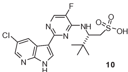
(S)-2-((2-(5-chloro-1H-pyrrolo[2,3-b]pyridin-3-yl)-5-fluoropyrimidin-4-yl)amino)-3,3-dimethylbutane-1-sulfonic acid (10)
