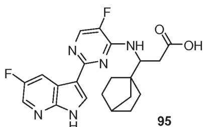
(+/-)-3-(Bicyclo[2.2.1]heptan-1-yl)-3-(5-fluoro-2-(5-fluoro-1H-pyrrolo[2,3-b]pyridin-3-yl)pyrimidin-4-yl)amino)propanoic acid (95)
