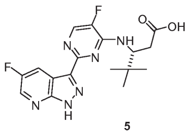
( R )-3-(((5-fluoro-2-(5-fluoro-1 H -pyrazolo[3,4- b ]pyridin-3-yl)pyrimidin-4-yl)amino)-4,4-dimethylpentanoic acid (5)
