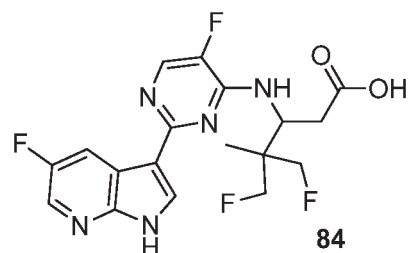
(+/-)-5-Fluoro-3-((5-fluoro-2-(5-fluoro-1H-pyrrolo[2,3-b]pyridin-3-yl)pyrimidin-4-yl)amino)-4-(fluoromethyl)-4-methylpentanoic acid (84)
