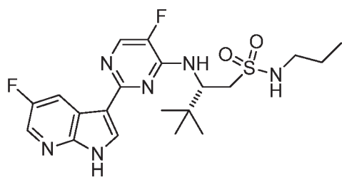
(S)-2-(5-Fluoro-2-(5-fluoro-1H-pyrrolo[2,3-b]pyridin-3-yl)pyrimidin-4-ylamino)-3,3-dimethyl-N-propylbutane-1-sulfonamide (34)
