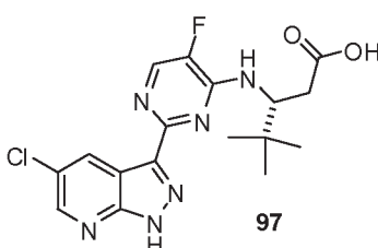
( R )-3-(((2-(5-chloro-1 H -pyrazolo[3,4- b ]pyridin-3-yl)-5-fluoropyrimidin-4-yl)amino)-4,4-dimethylpentanoic acid (97) and methylester (96)
