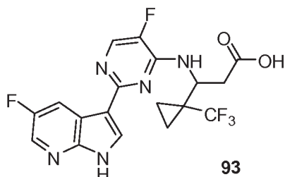
(+/-)-3-((5-Fluoro-2-(5-fluoro-1H-pyrrolo[2,3-b]pyridin-3-yl)pyrimidin-4-yl)amino)-3-(1-(trifluoromethyl)cyclopropyl)propanoic acid (93)
