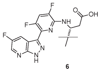
( R )-3-(((3,5-difluoro-6-(5-fluoro-1 H -pyrazolo[3,4- b ]pyridin-3-yl)pyridin-2-yl)amino)-4,4-dimethylpentanoic acid (6)
