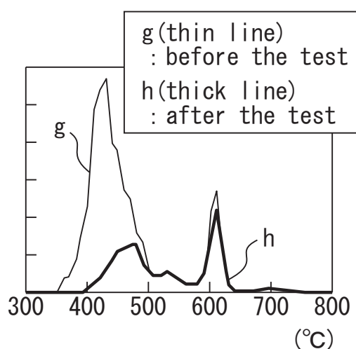
(2) GCD curve of the lubricant composition of Reference Example 2
