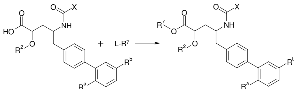
Scheme II
