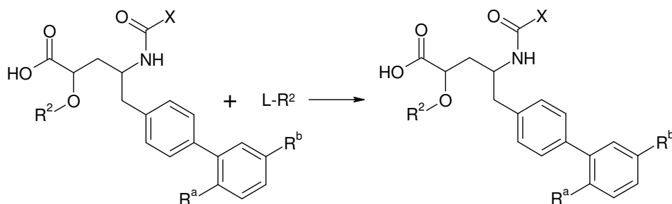
Scheme III
