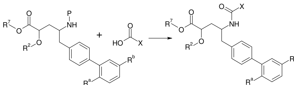
Scheme IV
