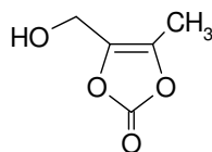
Scheme II
