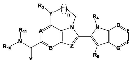
Formula (II)
