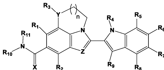
Formula (III)
