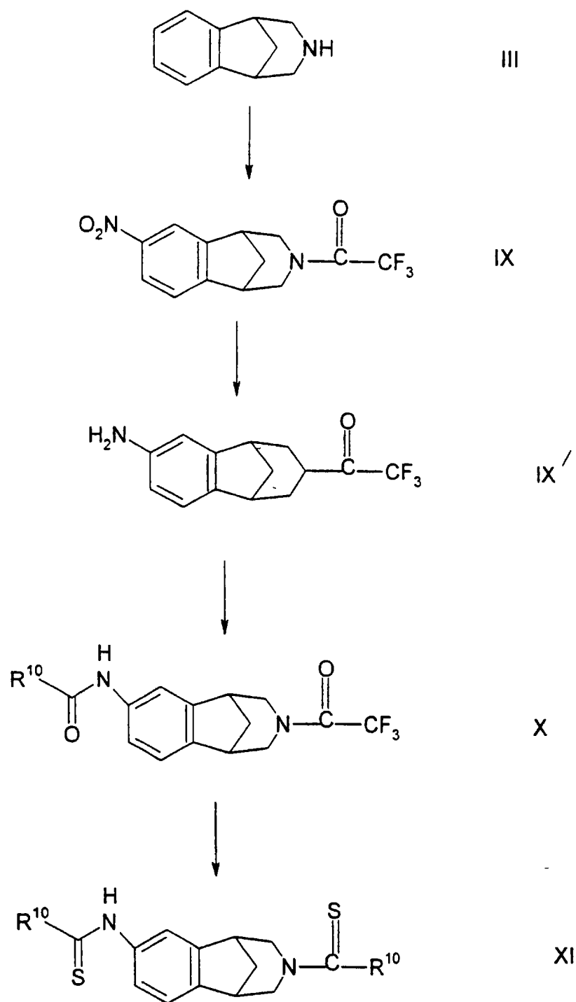
Scheme 6
