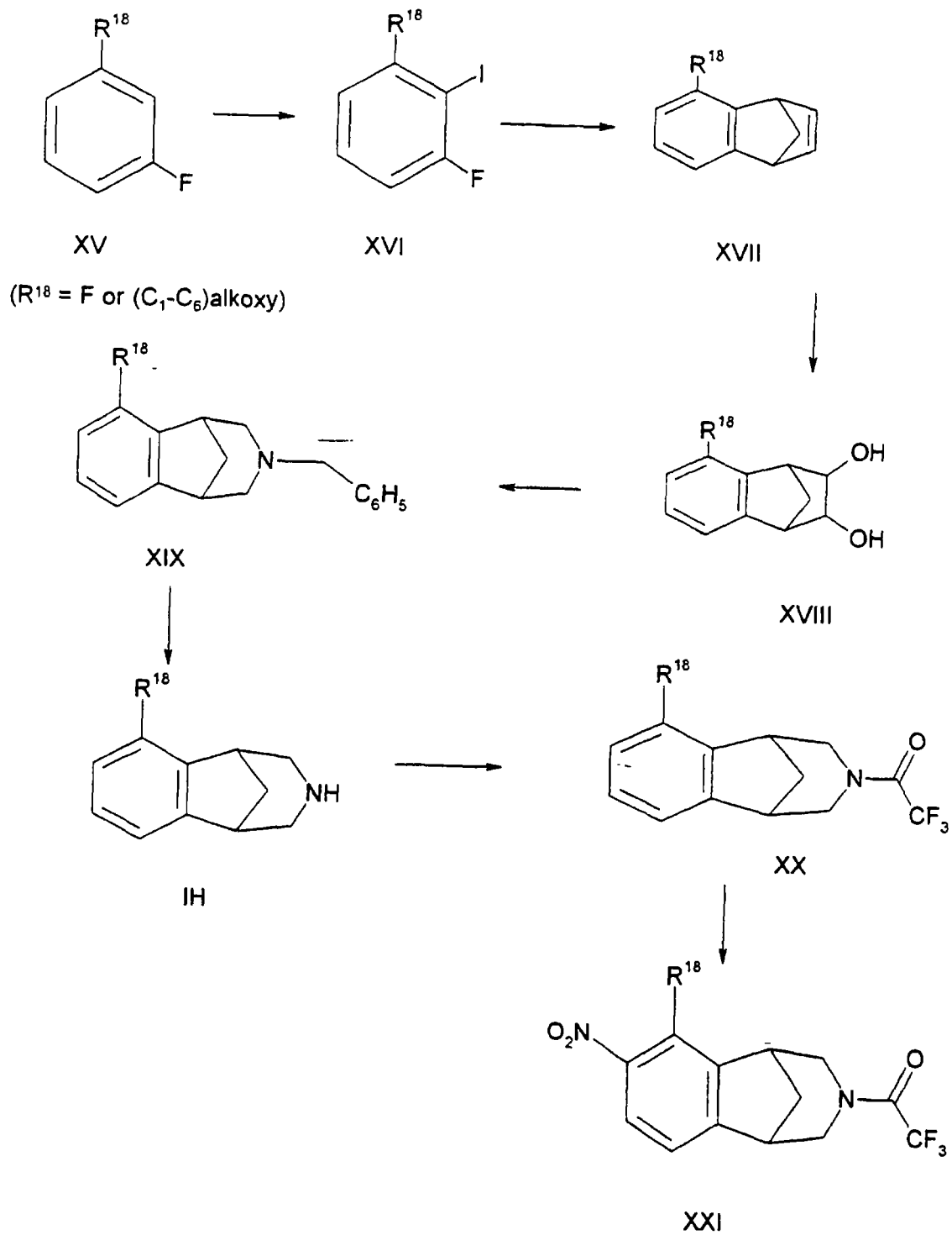
Scheme 8
