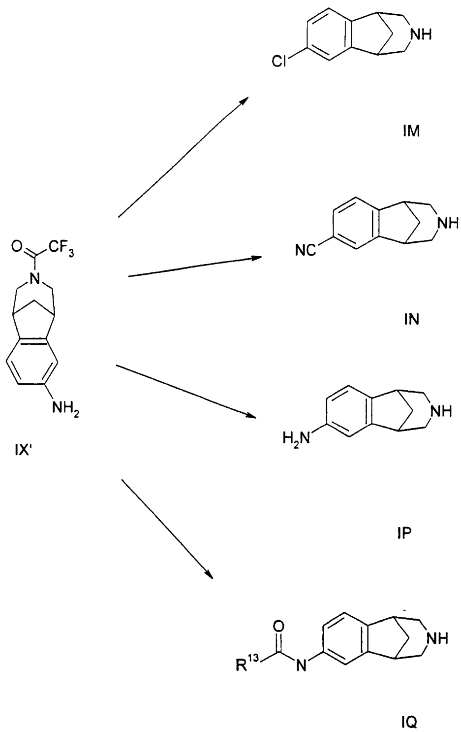
Scheme 10
