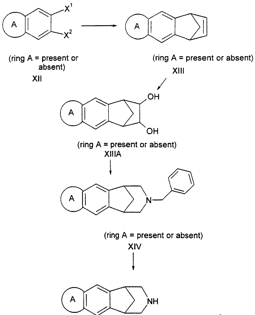
Scheme 7
