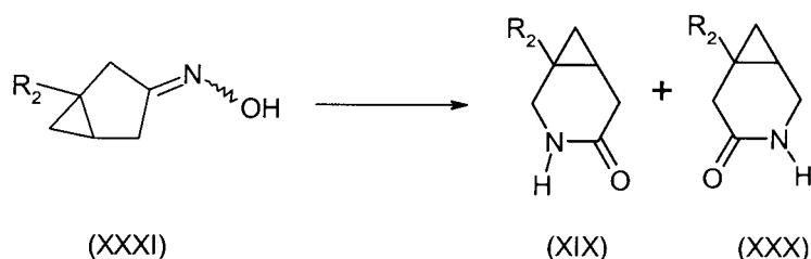
Scheme 30
