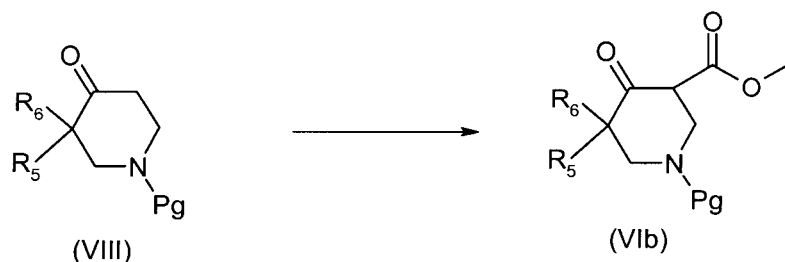
Scheme 13
