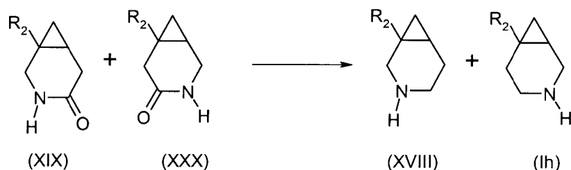
Scheme 29
