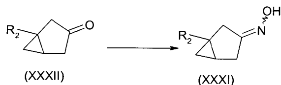
20 Scheme 31
