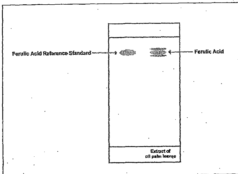
Figure 2: TLC Chromatogram of Ferulic Acid in extract of oil palm leaves
