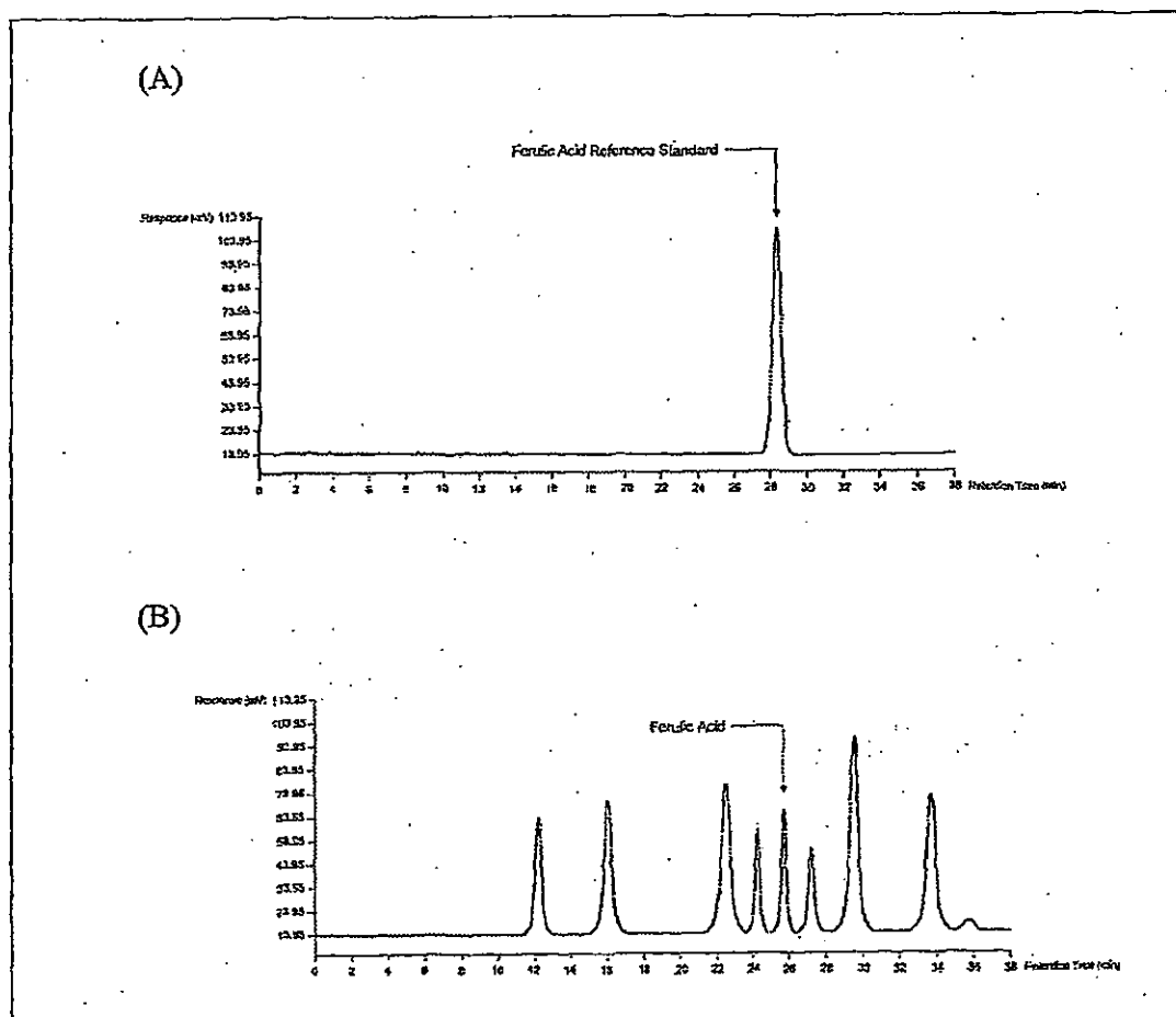
Figure 5: HPLC Chromatograms of (A) Ferulic Acid reference standard and (B) extract of oil palm leaves
