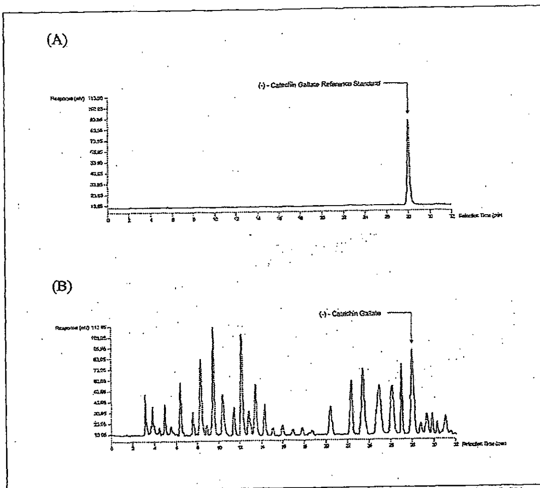
Figure 4: HPLC Chromatograms of (A) (-)-Catechin Gallate reference standard and (B) extract of oil palm leaves
