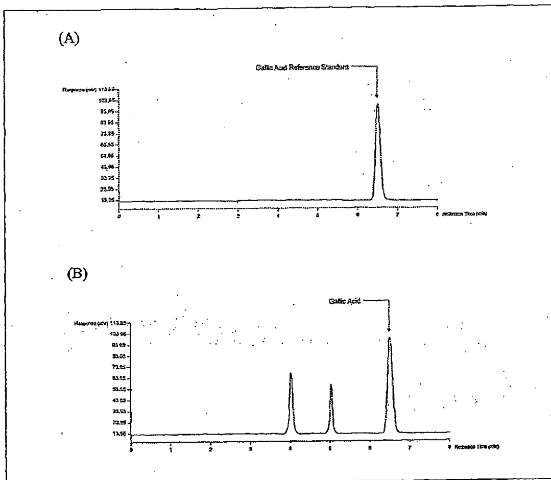
Figure 3: HPLC Chromatograms of (A) Gallic Acid reference standard and (B) extract of oil palm leaves
