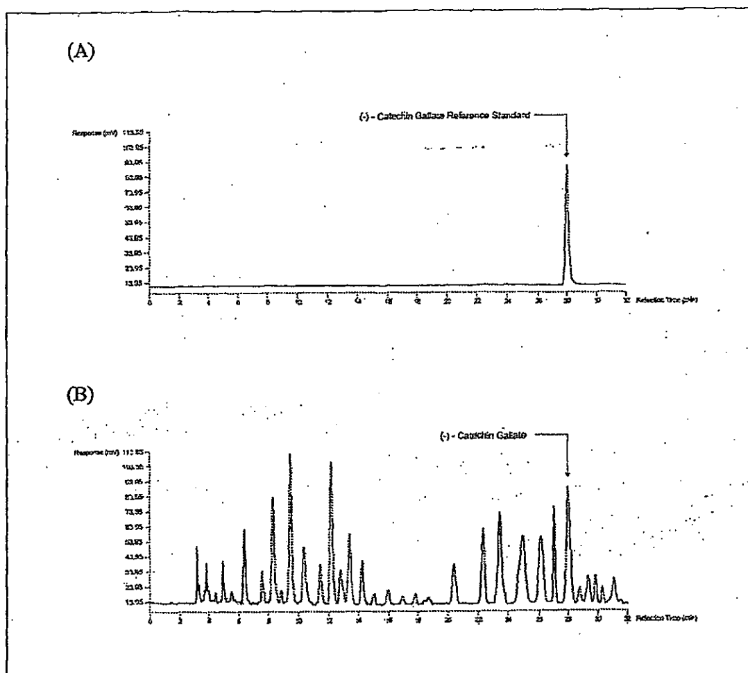
Figure 1: HPLC Chromatograms of (A) (-)-Catechin Gallate reference standard and (B) extract of oil palm leaves
