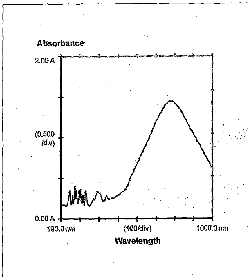
Figure 6: UV Chromatogram of Total Phenolic Acids in extract of oil palm leaves
