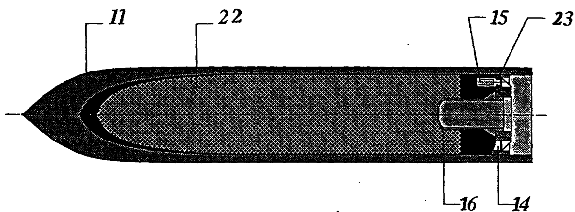
FIGURE 3: TYPICAL PENETRATING WARHEAD
