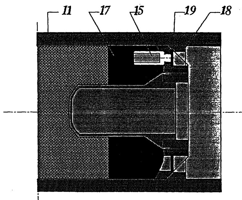
FIGURE 4: PENETRATING WARHEAD, REAR PART
