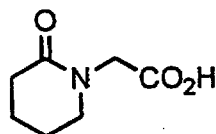
1-Carboxymethyl-2-piperidone
