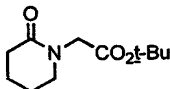
1- t -Butoxycarbonylmethyl-2-piperidone
