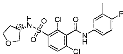
Compound 125
