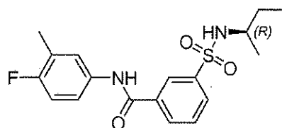
Compound 98
