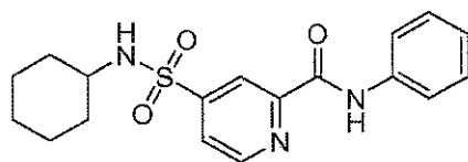
20 Compound 67
