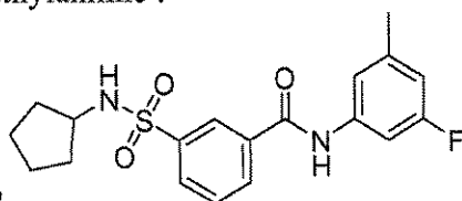
Compound 12
