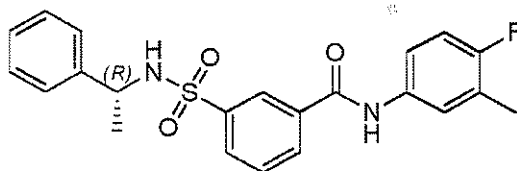
Compound 166
