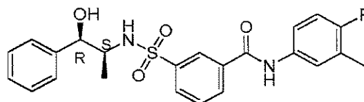
Compound 143
