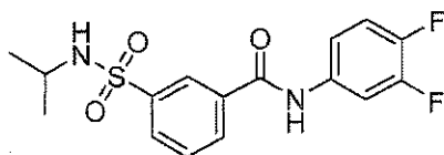
Compound 88
