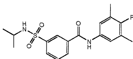
Compound 186
