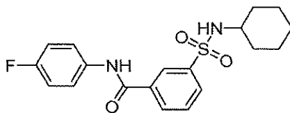
Compound 6
