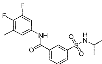
Compound 99
