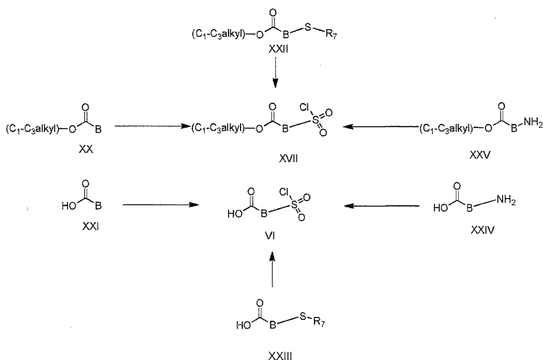
Scheme 7
