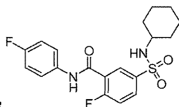
Compound 18
