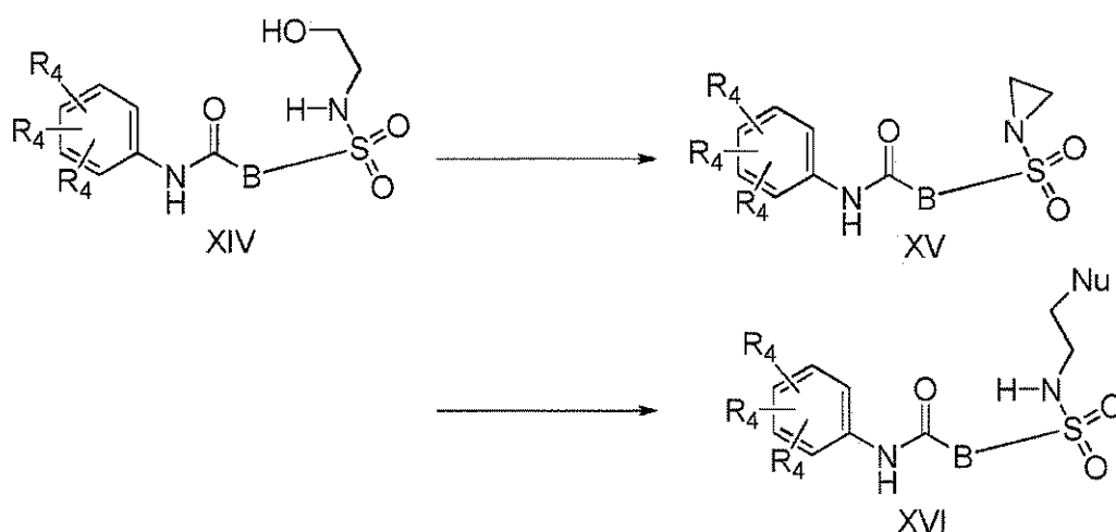
Scheme 5
