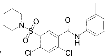
Compound 17
