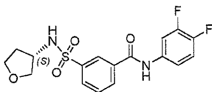
Compound 90
