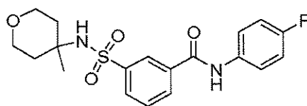
Compound 83
