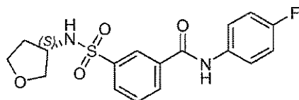
Compound 9
