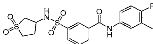
5 Compound 140
