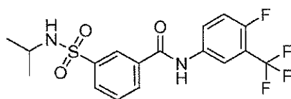
Compound 74
