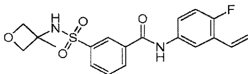
Compound 110
