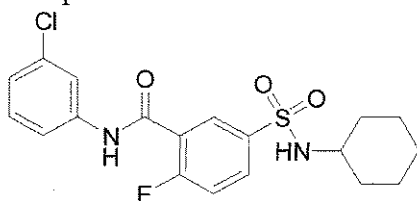
Compound 43
