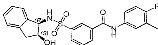
Compound 136
