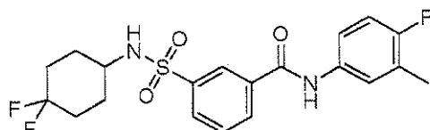
5 Compound 149
