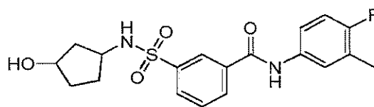
Compound 145
