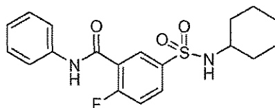
Compound 19
