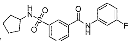
Compound 77
