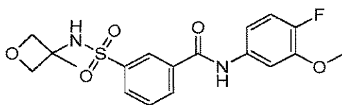
Compound 109
