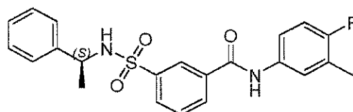
Compound 167
