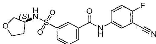
Compound 105
