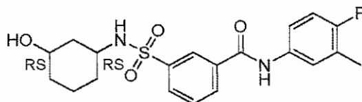
Compound 134
