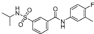
Compound 73
