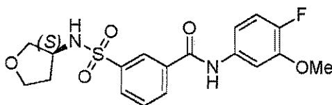
Compound 103
