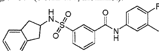
Compound 168
