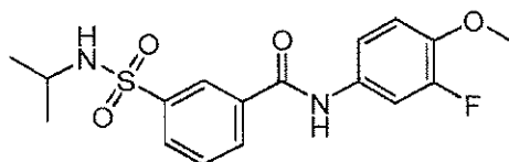
Compound 114
