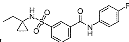
Compound 87
