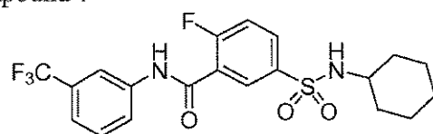
Compound 7
