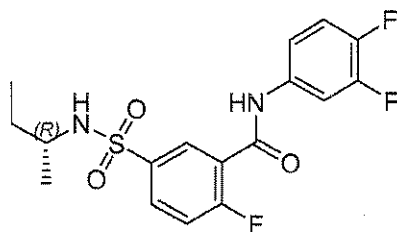
Compound 100
