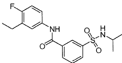
Compound 92
