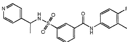
Compound 161
