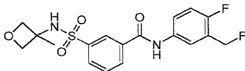
Compound 127
