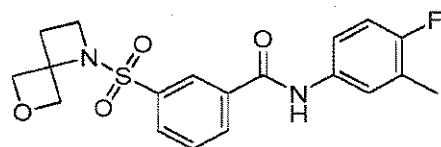
Compound 147
