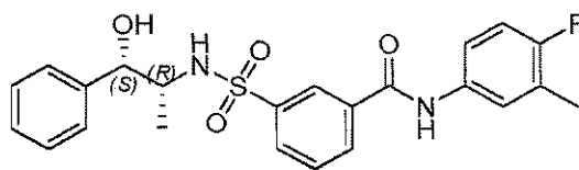
Compound 144
