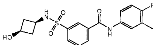
Compound 184b
