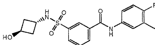
Compound 184a
