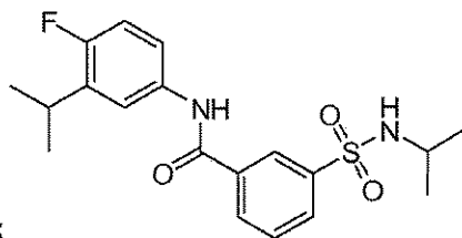
Compound 95
