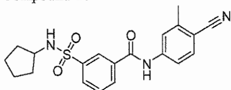
Compound 16
