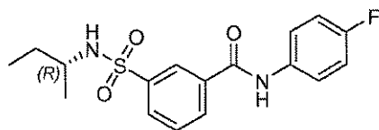
25 Compound 70
