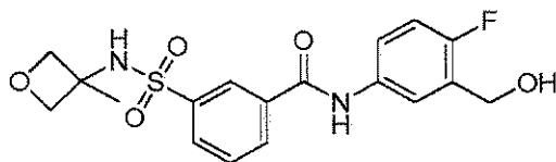
Compound 111
