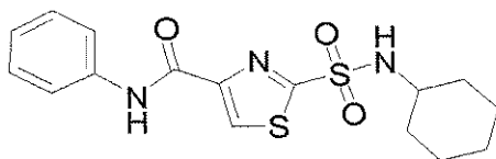
Compound 64
