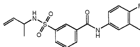
Compound 150
