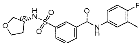
Compound 129
