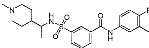
Compound 164
