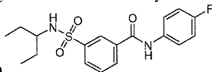
Compound 10
