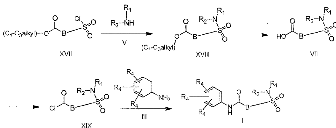
Scheme 6
