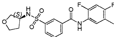
Compound 106
