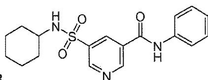
Compound 68
