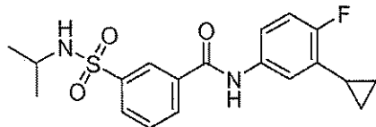
Compound 84
