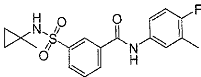
Compound 94
