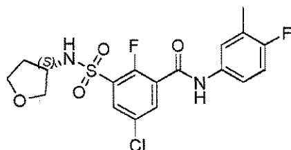
Compound 123
