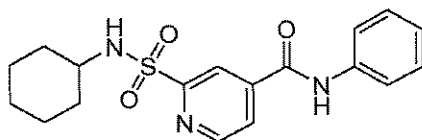
Compound 66
