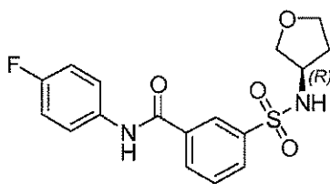
Compound 8
