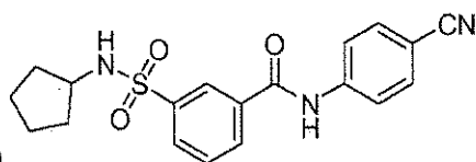
Compound 80
