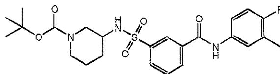
Compound 155
