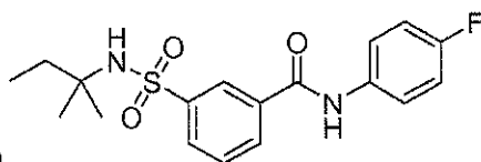
Compound 79
