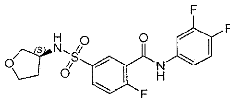
Compound 101
