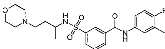
Compound 165
