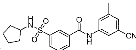
Compound 82
