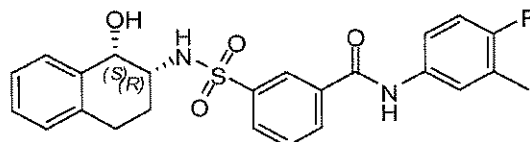
Compound 137
