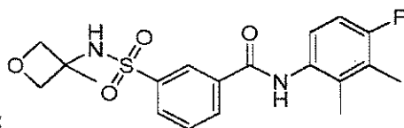
Compound 115
