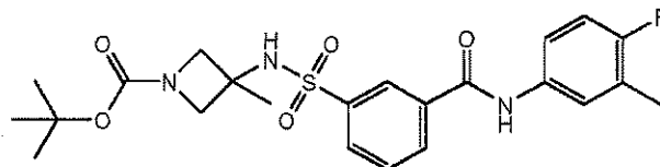
Compound 154
