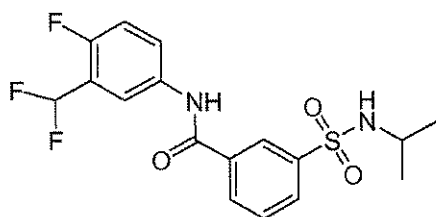
Compound 96
