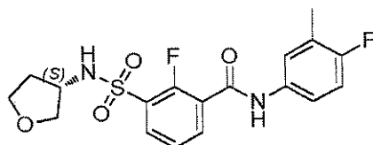
Compound 112
