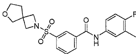
Compound 146
