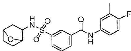
Compound 128
