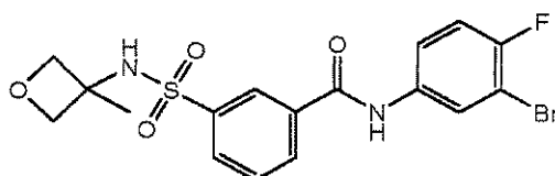
Compound 160
