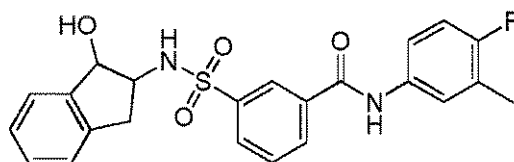
15 Compound 141
