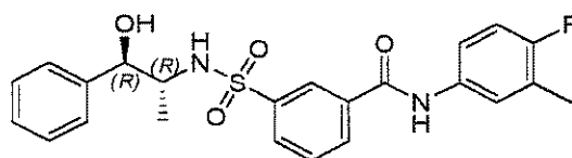
15 Compound 142
