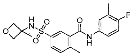
Compound 122
