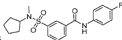
Compound 46
