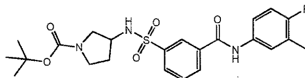
Compound 156
