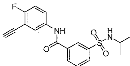
Compound 91
