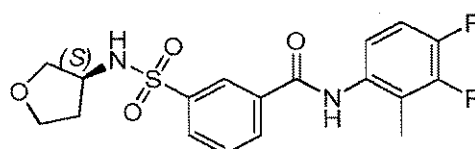
Compound 118
