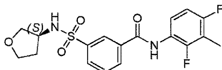
Compound 104
