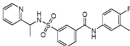
Compound 163
