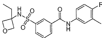
Compound 93
