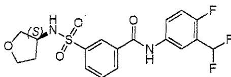
Compound 102
