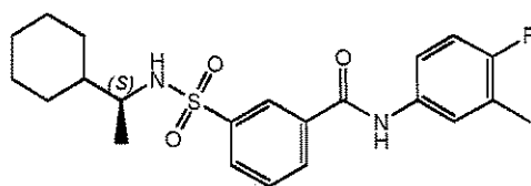
Compound 148
