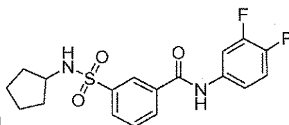
Compound 14
