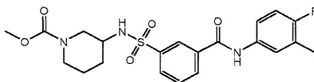
Compound 159
