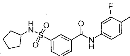
Compound 13
