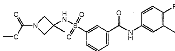
Compound 157
