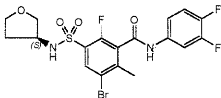
Compound 187
