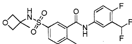
Compound 113
