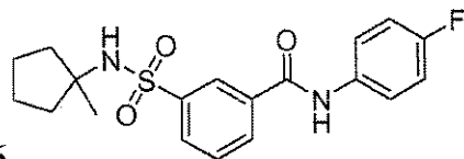
20 Compound 76
