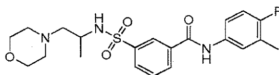
Compound 117
