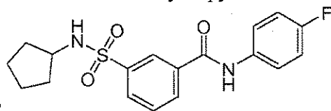
Compound 2
