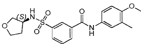
Compound 107
