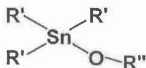
[Chemical Formula 71]
