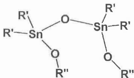
[Chemical Formula 71]
