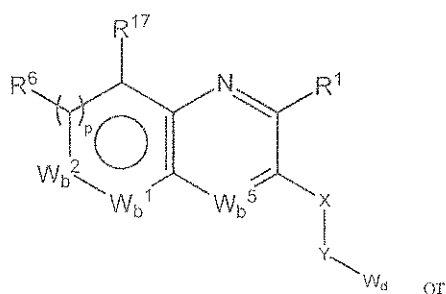
Formula (X)
