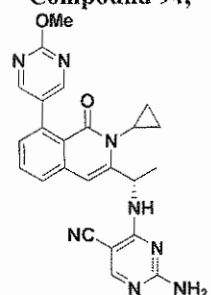
Compound 105,
