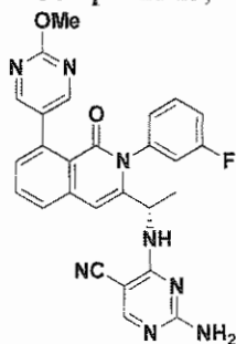
Compound 22,
