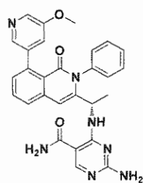
Compound 10,
