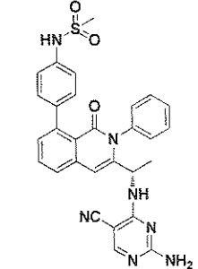
Compound 167,
