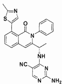
Compound 68,
