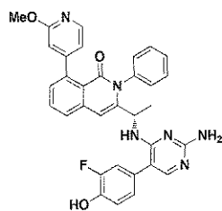
Compound 159,
