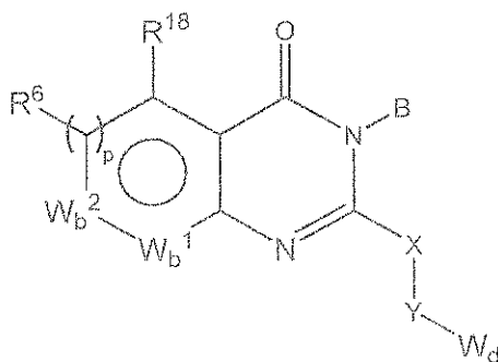
Formula (XV)
