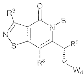
Formula (V).
