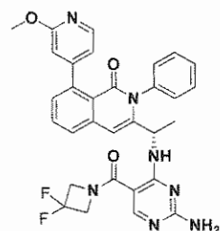
Compound 432,
