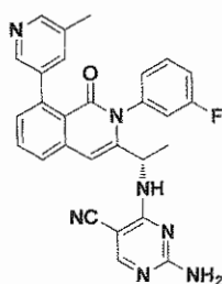
Compound 26,
