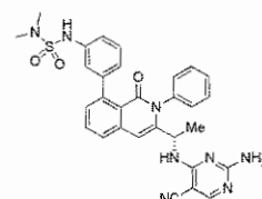
Compound 127,
