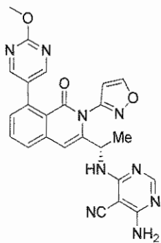
Compound 337,
