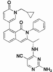
Compound 232,
