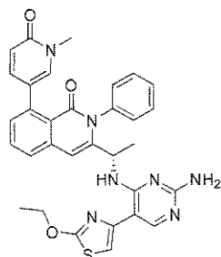
Compound 138,
