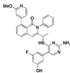
Compound 161,
