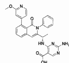
Compound 111,
