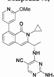
Compound 107,
