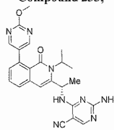
Compound 327,
