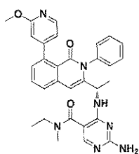
Compound 155,
