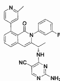
Compound 24,
