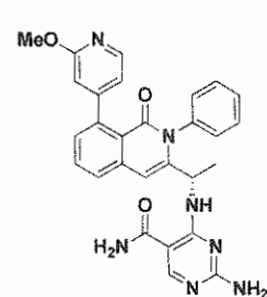
Compound 446,
