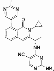
Compound 445,
