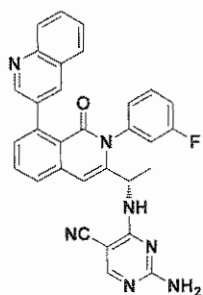
Compound 23,
