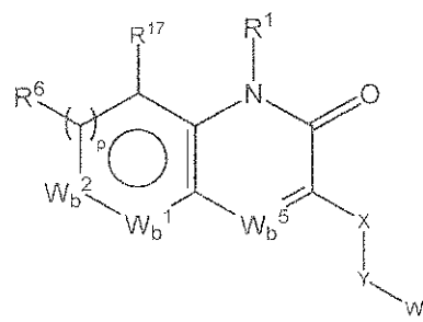
Formula (XI)
