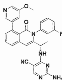
Compound 27,
