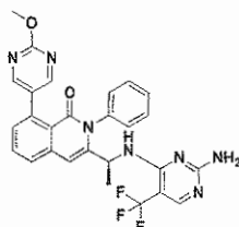
Compound 12,
