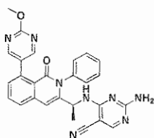
Compound 5,
