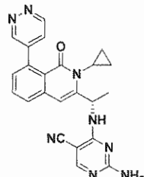
Compound 440,
