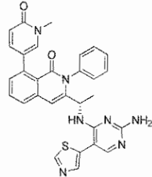
Compound 387,
