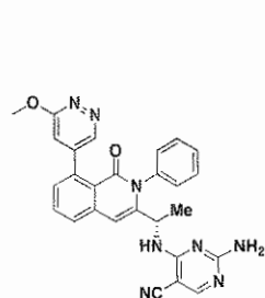
Compound 444,
