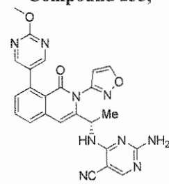
Compound 333,
