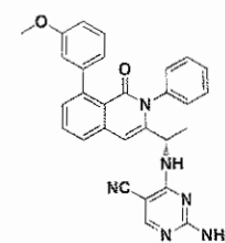
Compound 36,
