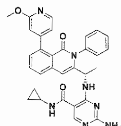
Compound 441,
