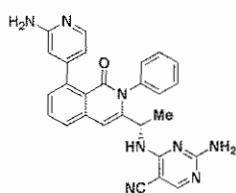
Compound 187,
