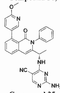
Compound 35,
