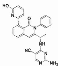
Compound 205,
