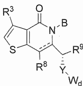
Formula (VII).
