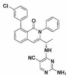
Compound 34,
