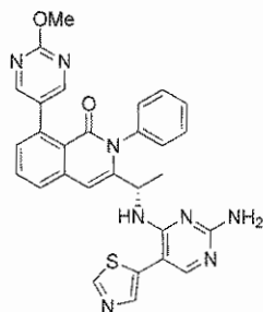
Compound 389,
