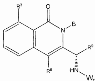
Formula (IIIb-1).
