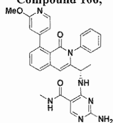
Compound 113,
