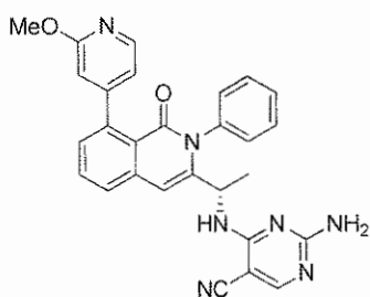
Compound 49,
