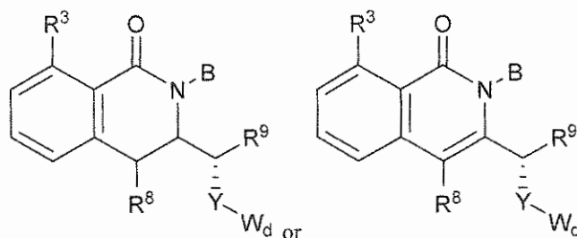
Formula (IIIa)
