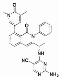
Compound 231,
