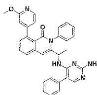
Compound 179,
