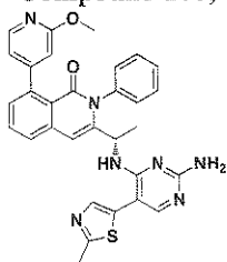
Compound 181,
