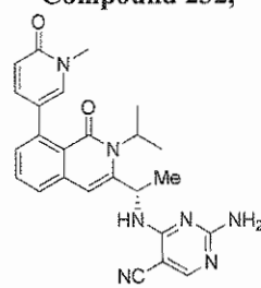
Compound 326,
