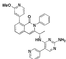
Compound 133,
