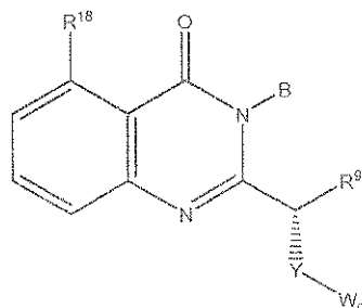
Formula (XVII).
