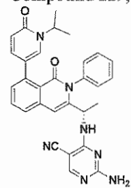
Compound 234,
