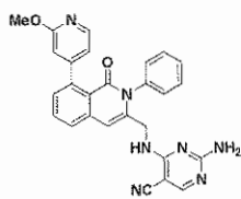
Compound 242,
