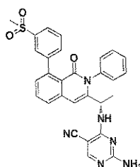
Compound 164,
