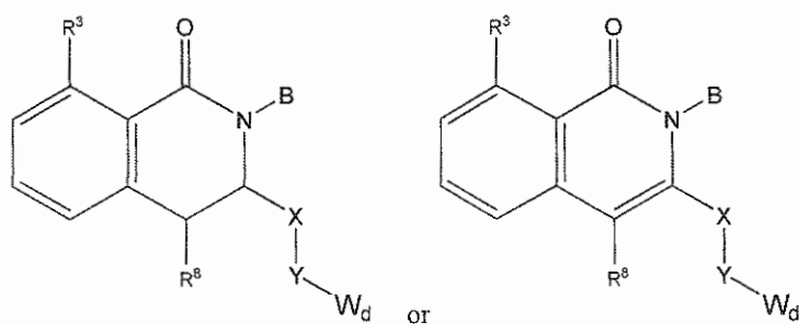
Formula (IIa)
