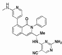
Compound 185,
