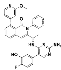
Compound 163,
