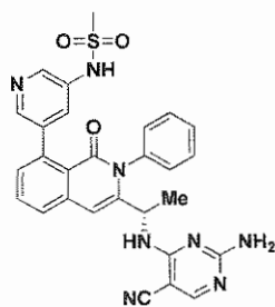
Compound 191,
