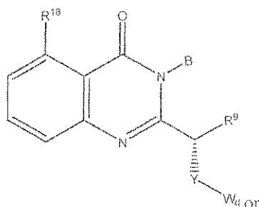
Formula (XVII).
