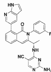
Compound 25,
