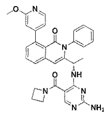
Compound 154,
