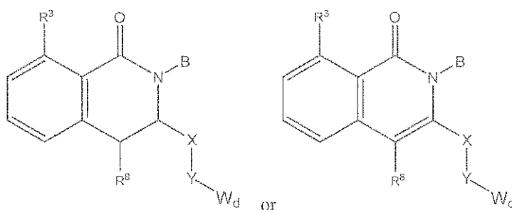
Formula (IIa)
