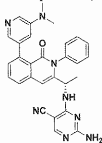
Compound 96,
