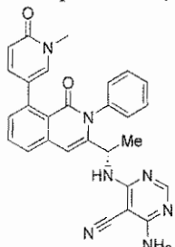
Compound 439,
