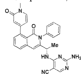
Compound 182,
