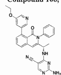
Compound 115,
