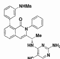
Compound 126,
