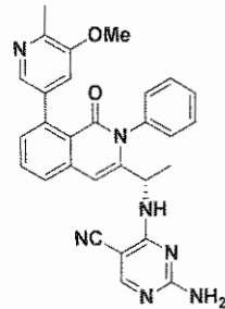
Compound 100,
