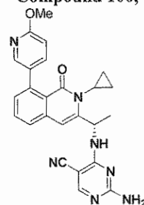
Compound 108,
