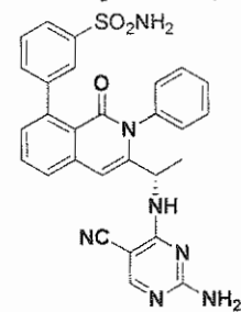
Compound 102,
