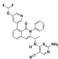
Compound 152,
