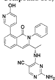
Compound 156,
