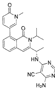
Compound 359,
