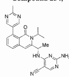
Compound 328,
