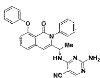
Compound 151,
