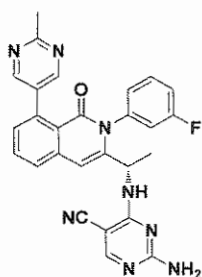
Compound 20,
