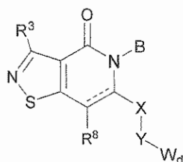
Formula (IV);
