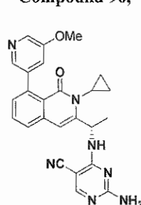
Compound 106,
