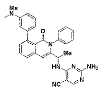
Compound 153,
