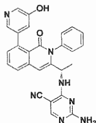
Compound 13,
