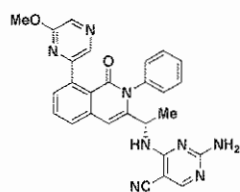
Compound 226,
