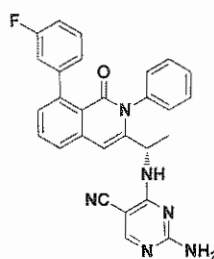
Compound 33,
