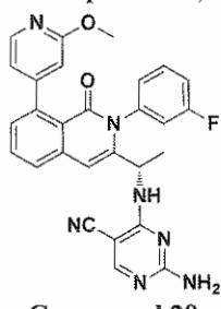
Compound 28,
