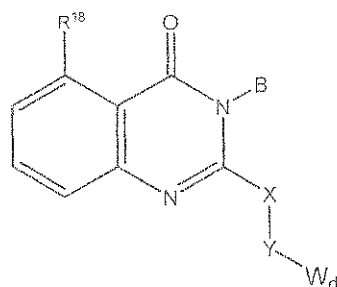
Formula (XVI).
