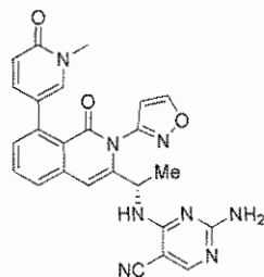
Compound 338,
