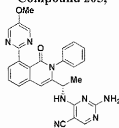
Compound 228,
