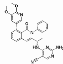
Compound 192,
