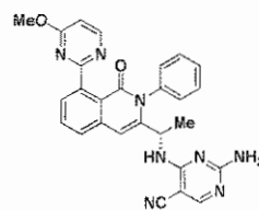
Compound 229,
