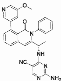
Compound 9,
