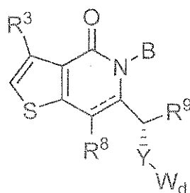
Formula (VII).
