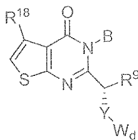
Formula (XXI).
