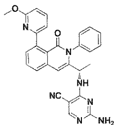
Compound 166,
