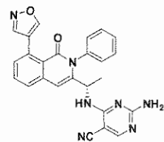
Compound 74,
