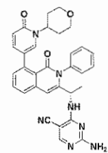
Compound 235,
