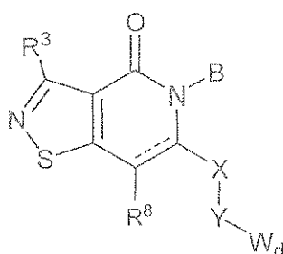
Formula (IV).
