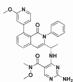
Compound 442,
