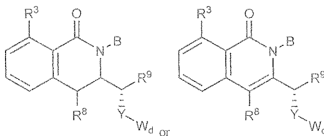
Formula (IIIa)
