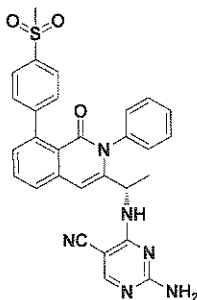
Compound 165,
