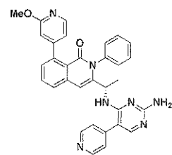
Compound 169,
