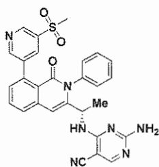
Compound 189,
