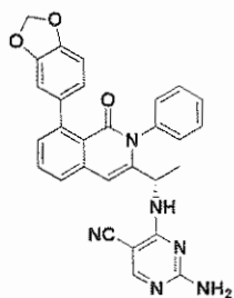
Compound 94,
