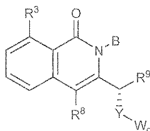
Formula (IIIb),
