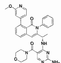
Compound 119,
