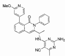
Compound 364,
