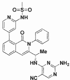
Compound 443,
