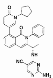
Compound 233,
