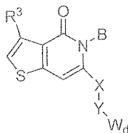
Formula (VIII).
