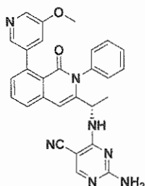
Compound 9,
