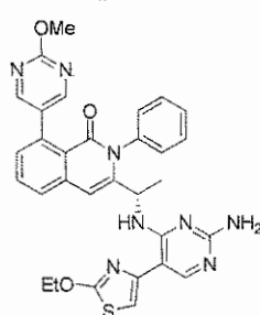
Compound 396,
