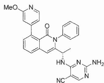
Compound 49,
