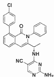
Compound 32,
