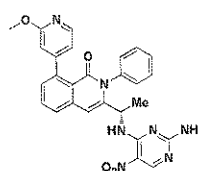
Compound 177,
