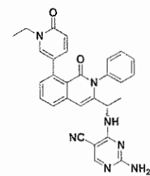
Compound 230,
