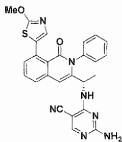
Compound 70,
