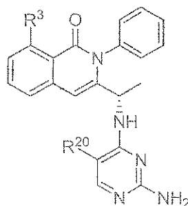
(XXIII)
