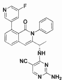
Compound 98,
