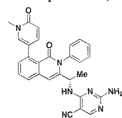
Compound 183,
