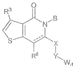
Formula (VI).
