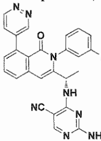
Compound 30,
