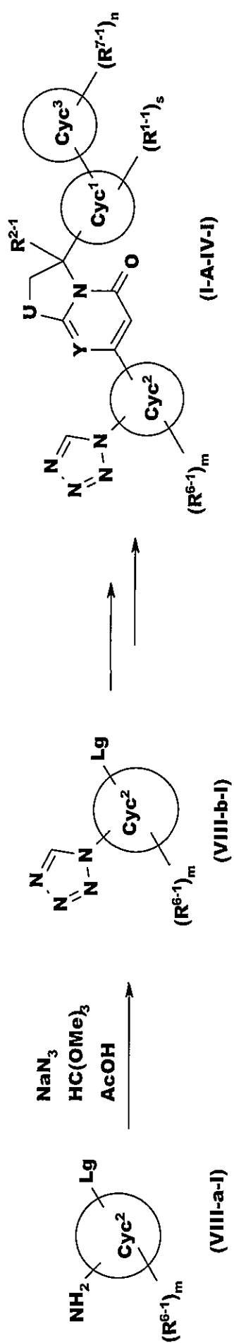
Reaction Scheme 12
