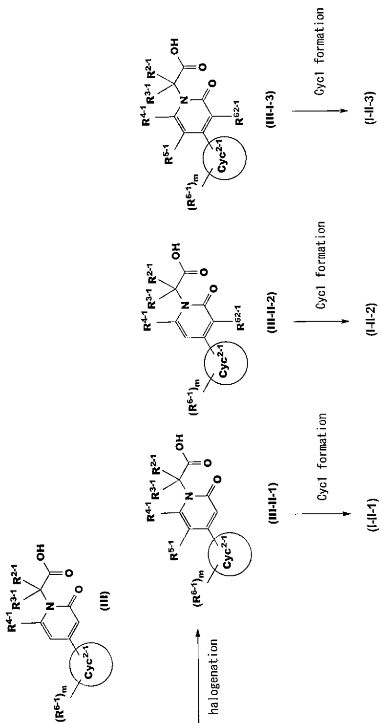
Reaction Scheme 19
