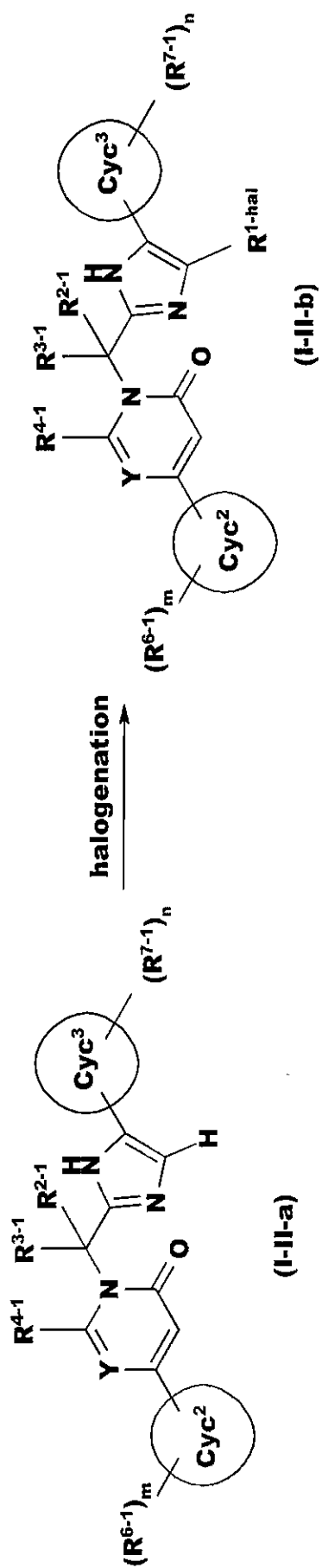
Reaction Scheme 2
