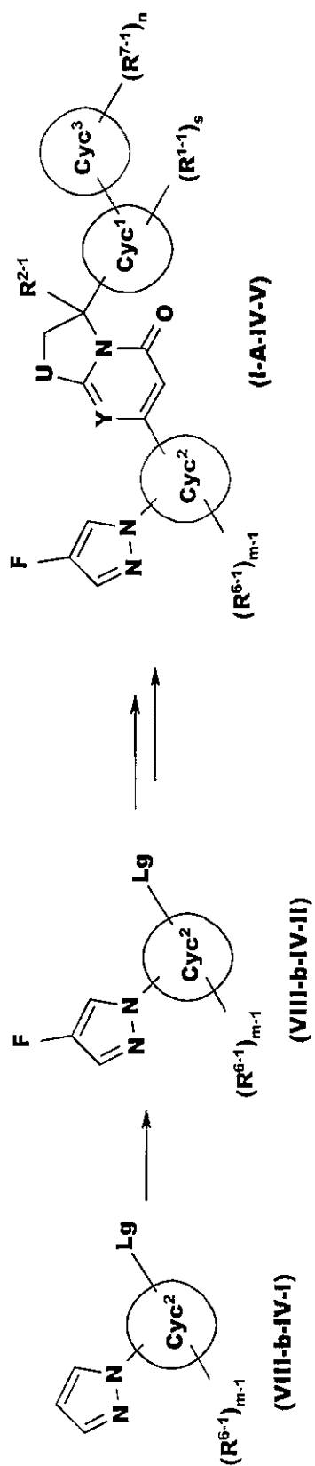
Reaction Scheme 16
