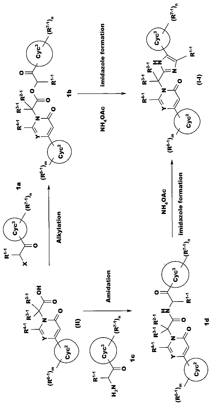
Reaction Scheme 1
