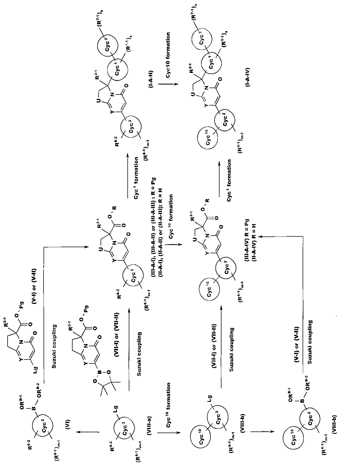
Reaction Scheme 11
