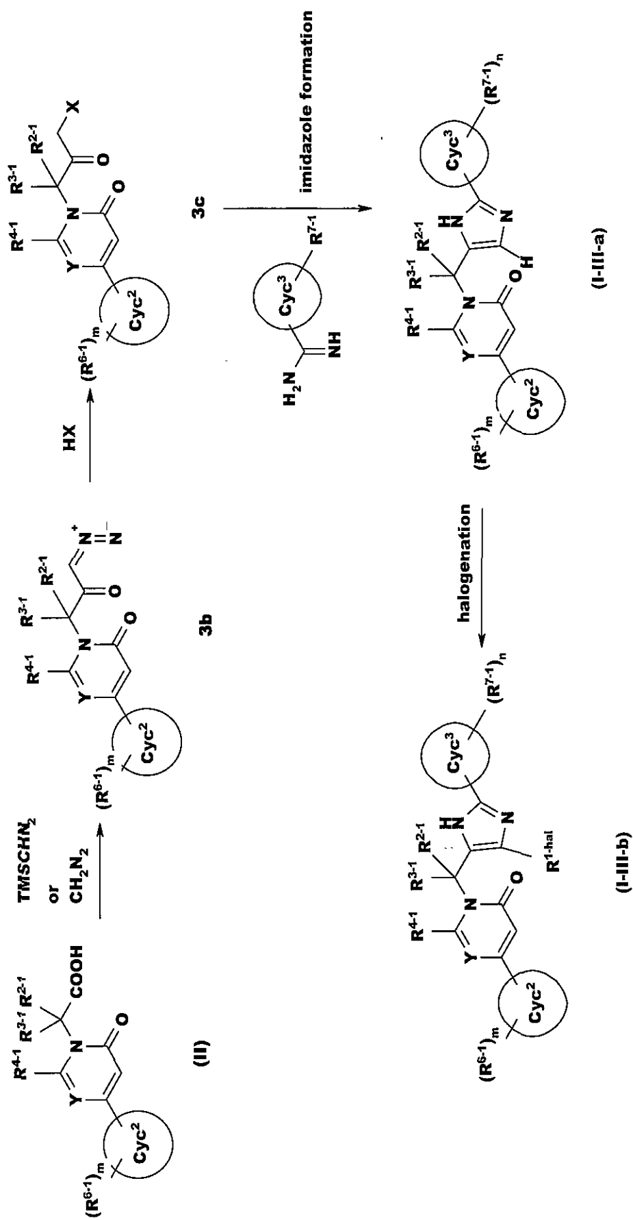
Reaction Scheme 3
