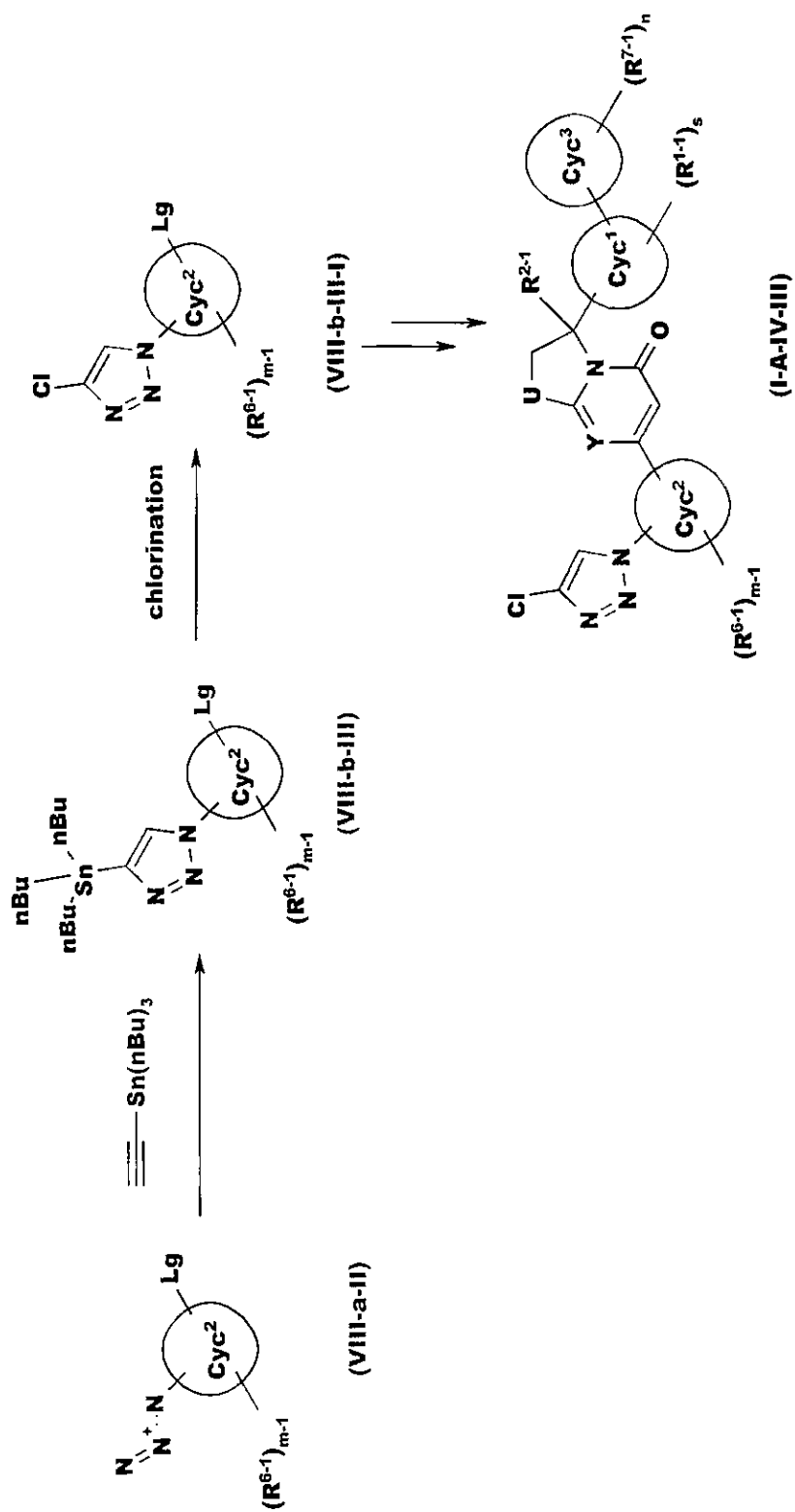
Reaction Scheme 14
