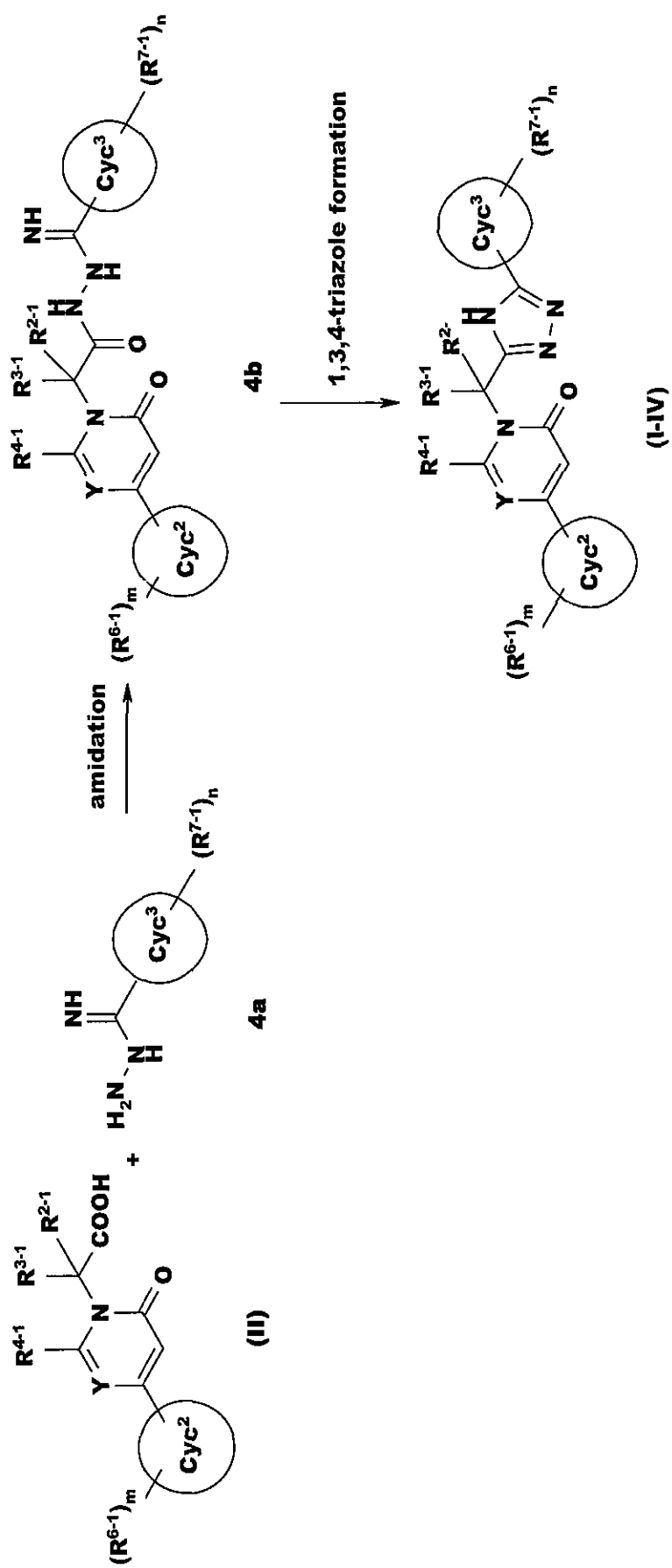
Reaction Scheme 4
