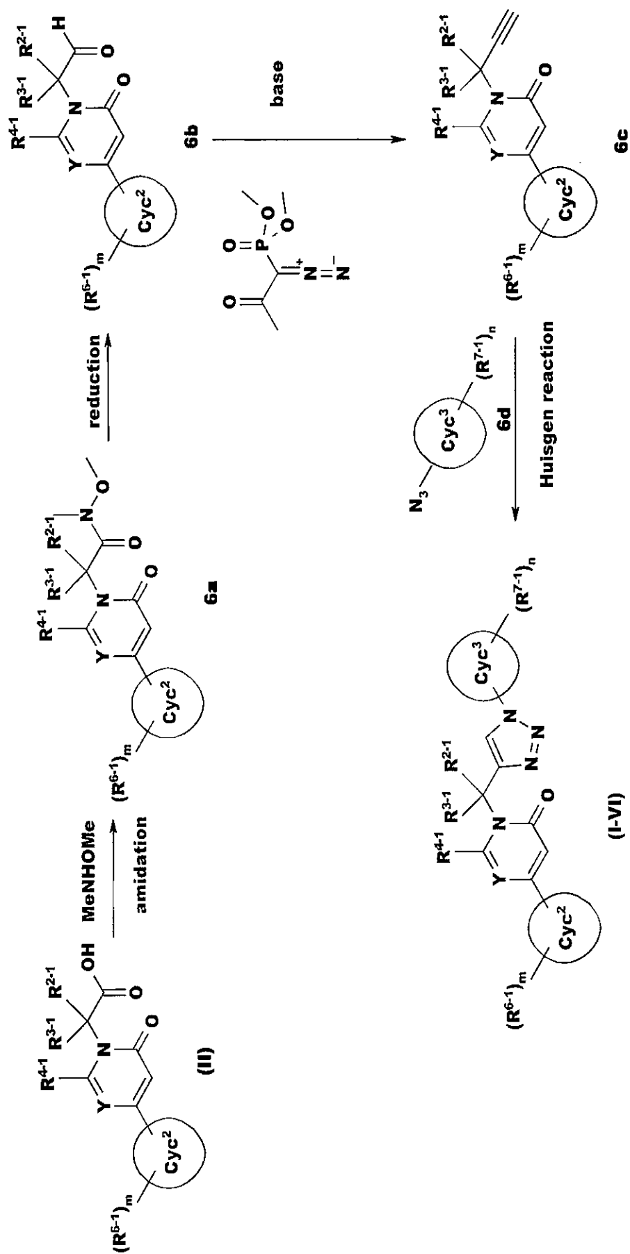
Reaction Scheme 6
