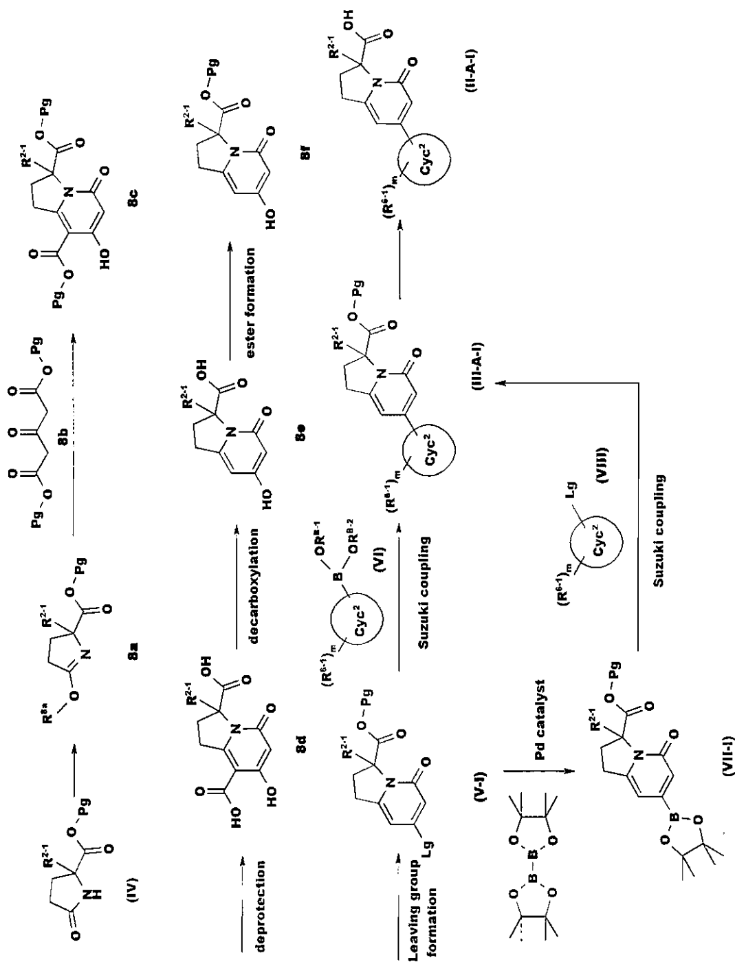
Reaction Scheme 8
