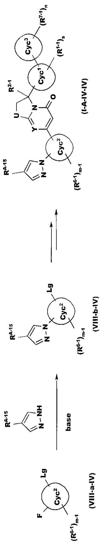
Reaction Scheme 15
