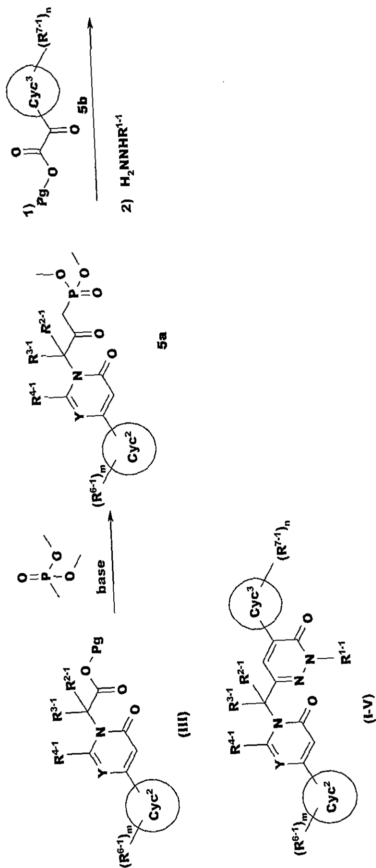
Reaction Scheme 5
