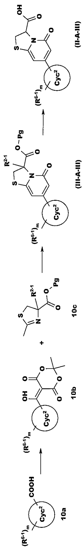
Reaction Scheme 10
