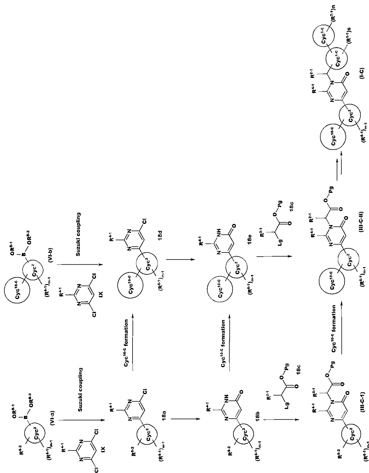
Reaction Scheme 18
