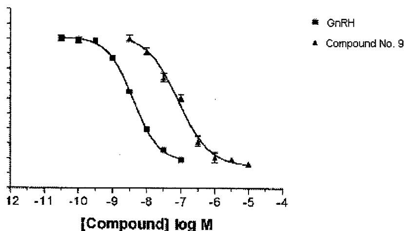
Figure 1. Effects of Compounds on ^{125}\text{I} -GnRH-A Binding to hGnRH Receptors in HEK-293 Cell Membranes
