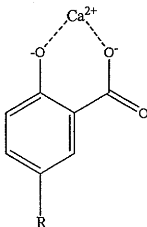
single aromatic ring hydrocarbyl salicylate
