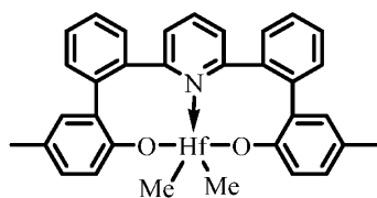
Catalyst 14
