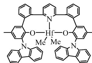
Catalyst 3
