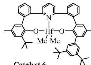
Catalyst 6
