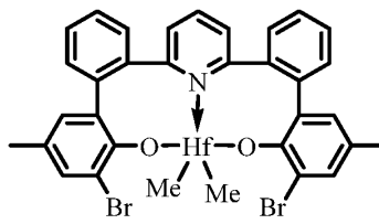
Catalyst 13
