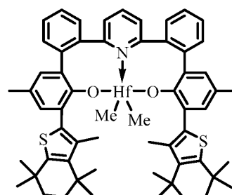
Catalyst 11
