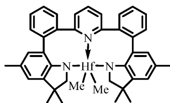
Catalyst 12
