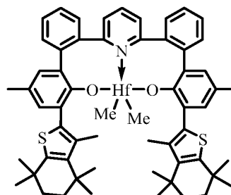
Catalyst 11
