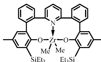
Catalyst 17
