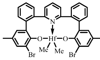
Catalyst 13
