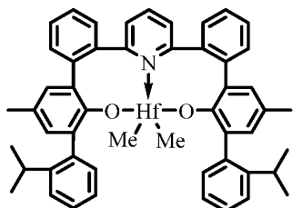
Catalyst 8
