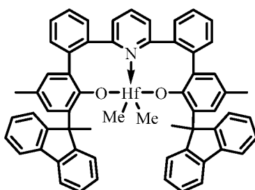
Catalyst 10
