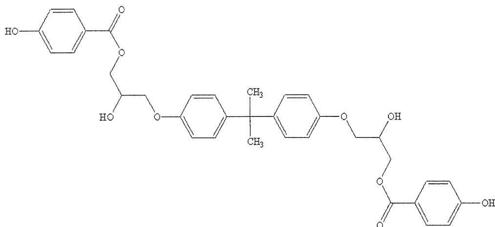
[Chemical Formula 19]
