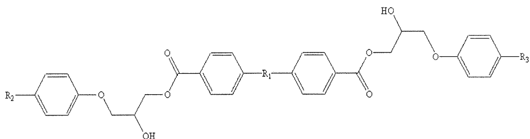
[Chemical Formula 14]
