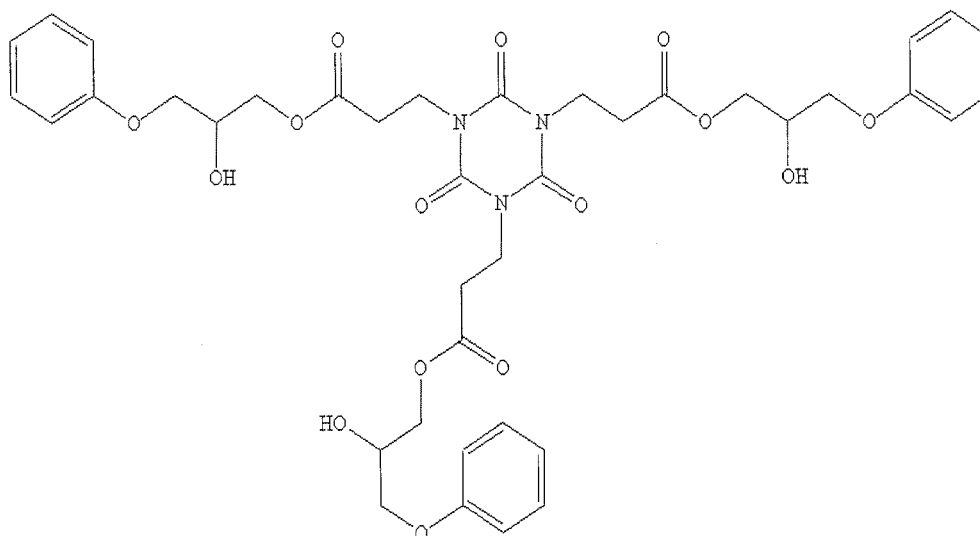
[Chemical Formula 20]
