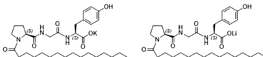
Compound I-5
