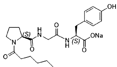
Compound I-7
