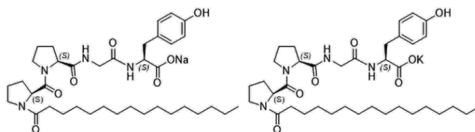
[Compound I-1]
