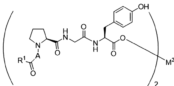
(Formula I-A)
