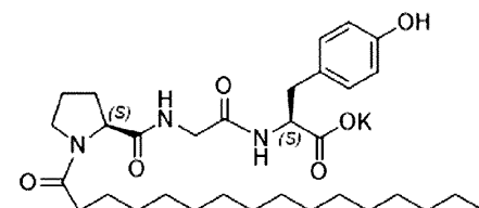
Compound I-5
