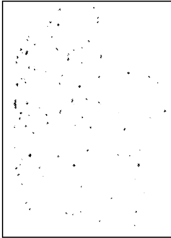
73 features
