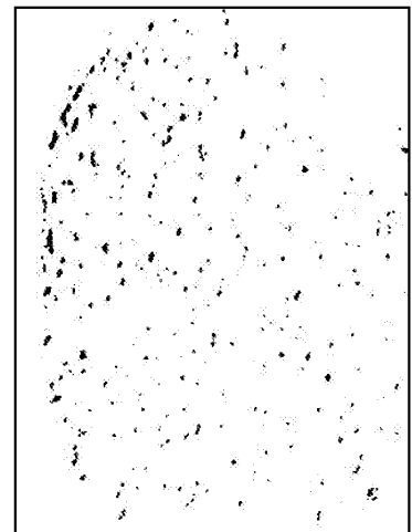
116 features
