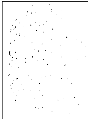
86 features
