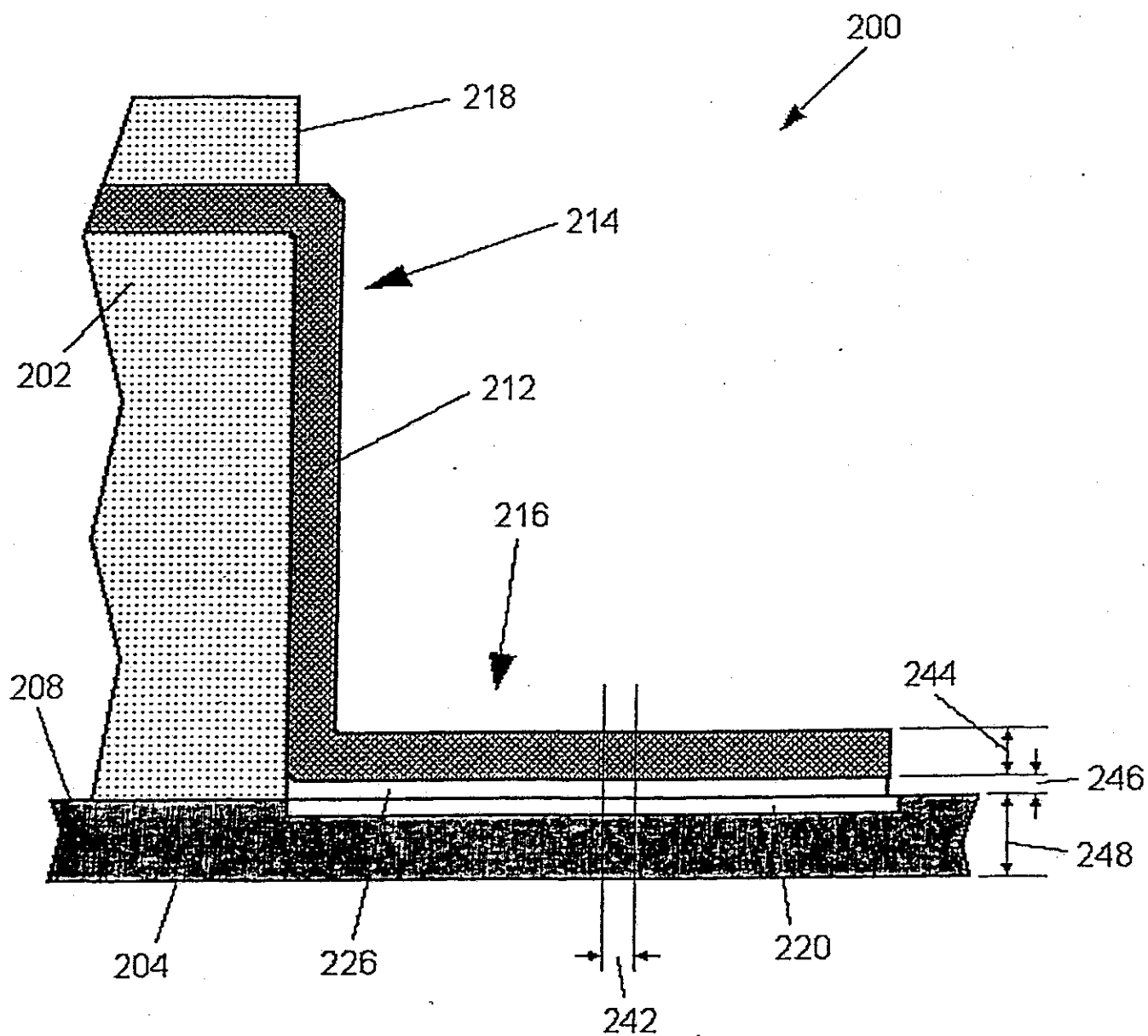
FIG. 11 Prior Art
