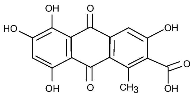
Kermesic acid
