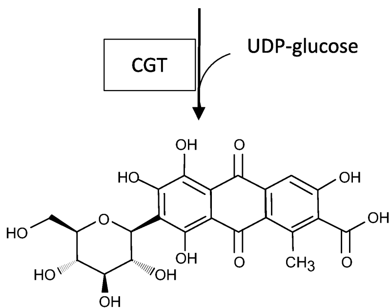
Carminic Acid
