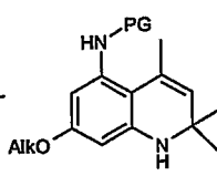
XXVII-a R 1 , R 2 = Me XXVII-b R 1 , R 2 = H
