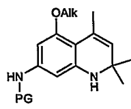
XXVI-a R 1 , R 2 = Me XXVI-b R 1 , R 2 = H
