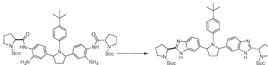
(2 S ,2' S )- tert -butyl 2,2'-(5,5'-(1-(4- tert -butylphenyl)pyrrolidine-2,5-diyl)bis(1 H -benzo[ d ]imidazole-5,2-diyl))dipyrrolidine-1-carboxylate
