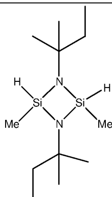
1,3-bis(tert-amyl)-2,4-dimethylcyclodisilazane
