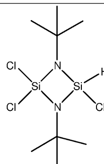
1,3-bis(tert-butyl)-2,2,4-trichloro- cyclodisilazane
