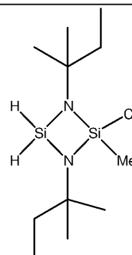
1,3-bis(tert-amyl)-2-chloro-2-methyl- cyclodisilazane
