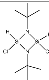
1,3-bis(tert-butyl)-2,4-dichlorocyclodisilazane
