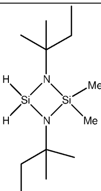
1,3-bis(tert-amyl)-2- dimethylcyclodisilazane
