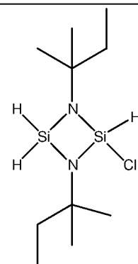
1,3-bis(tert-amyl)-2-chloro-cyclodisilazane
