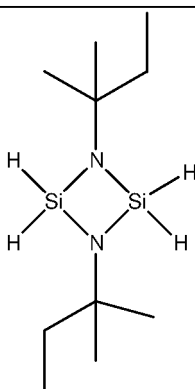
1,3-bis(tert-amyl)cyclodisilazane
