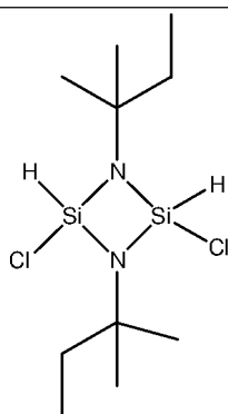
1,3-bis(tert-amyl)-2,4-dichloro- cyclodisilazane
