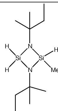
1,3-bis(tert-amyl)-2-methylcyclodisilazane
