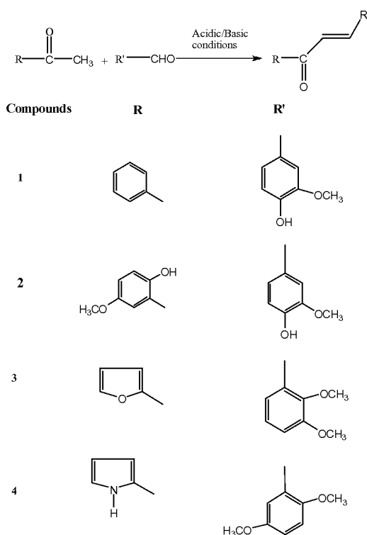
Synthesis of Chalcone 1 to 4
