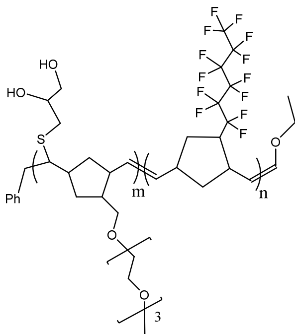
Poly(NTEG-b-NPF6)/Thioglycerol
