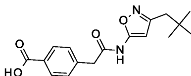
Preparation 117
