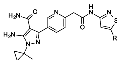
IIIf,
