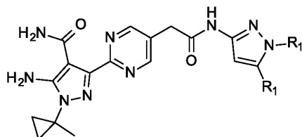
IIIq,
