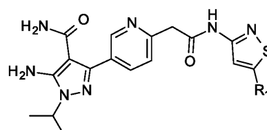
IIIf,
