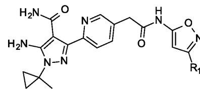
IIIi,
