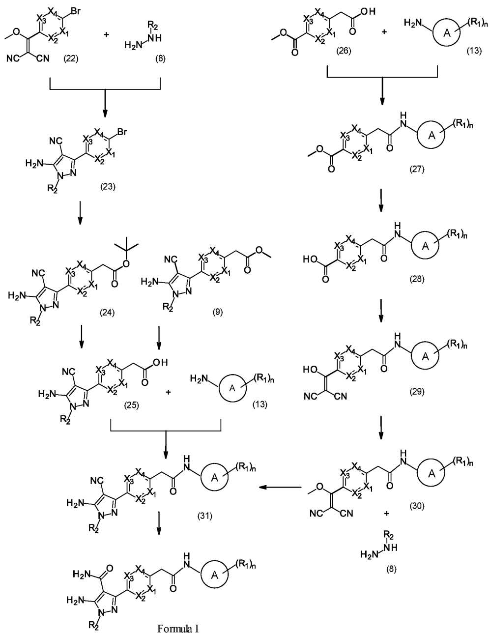
Scheme 4
