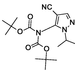
Preparation 91
