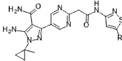
III n,
