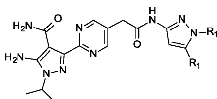
IIq,
