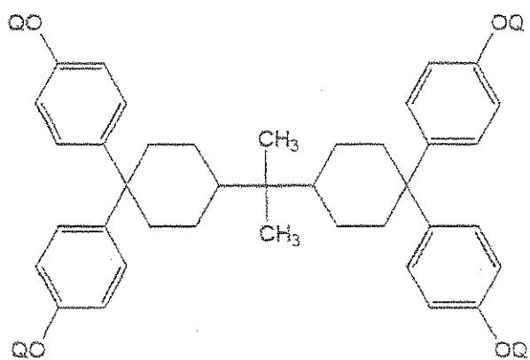
Quinone diazide compound (g)
