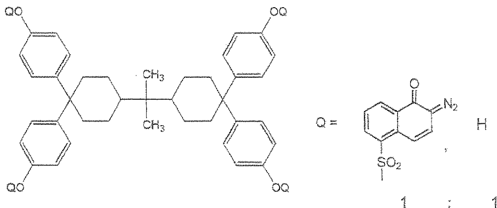
Quinone diazide compound (i)
