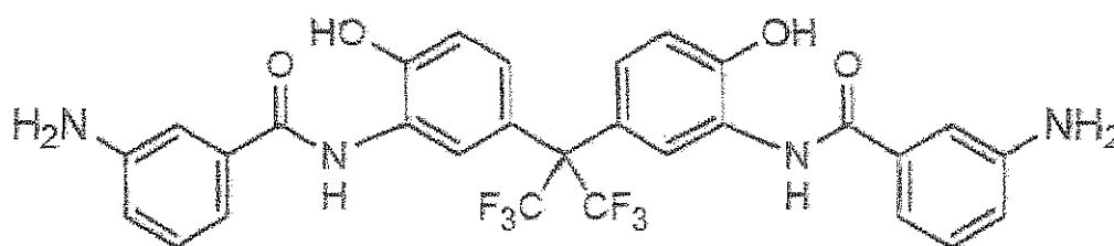
Hydroxyl group-containing diamine (b)
