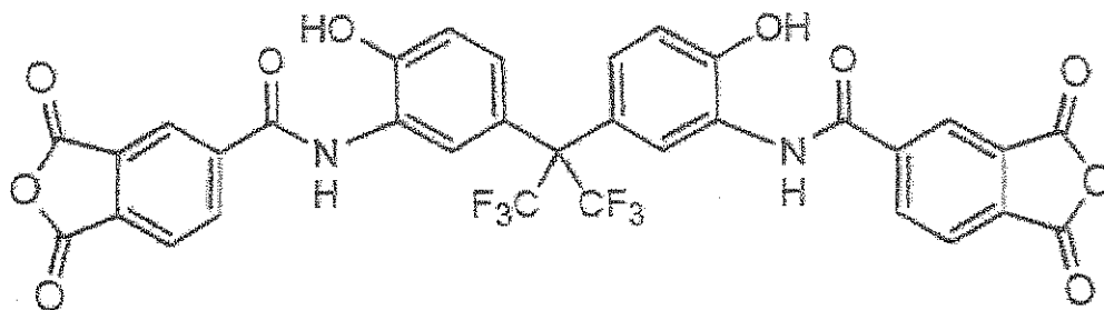
Hydroxyl group-containing acid anhydride (a)
