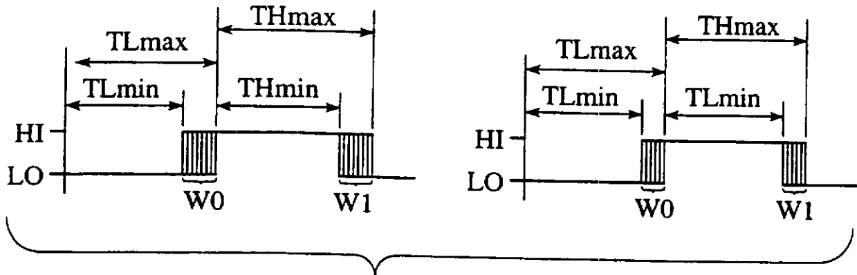
FIG. 1 (PRIOR ART)
