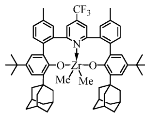
Complex 13
