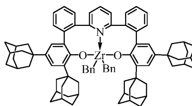
Complex 22
