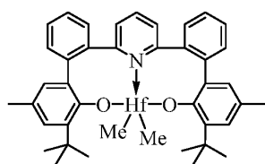
Complex 26
