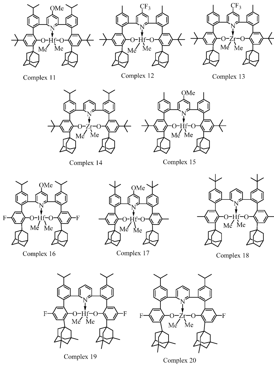
Scheme 3 (continued)
