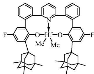
Complex 21
