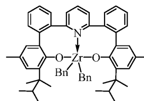
Complex 29
