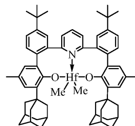
Complex 18
