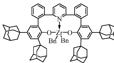
Complex 22
