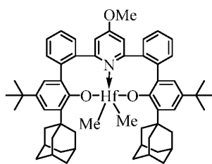
Complex 7
