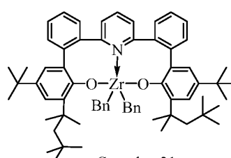
Complex 31
