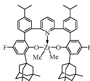
Complex 20
