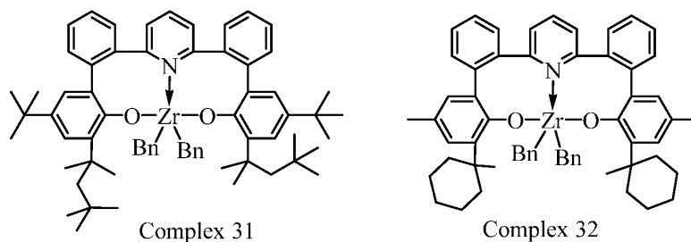
Scheme 3 (continued)
