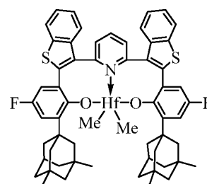
Complex 25
