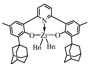
Complex 28 comparative
