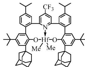
Complex 10
