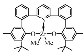
Complex 27
