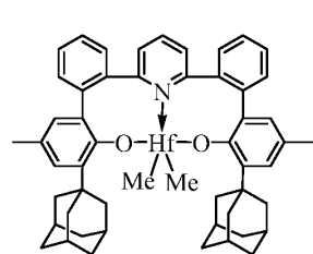
Complex 1
