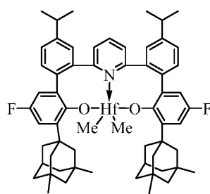
Complex 19
