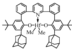
Complex 5
