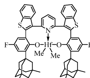
Complex 25
