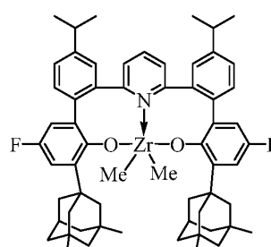
Complex 20
