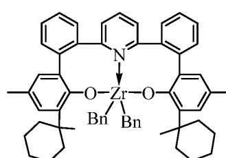
Complex 32
