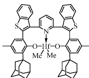
Complex 23
