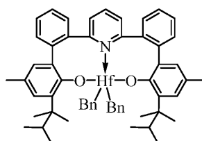
Complex 30
