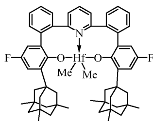
Complex 21
