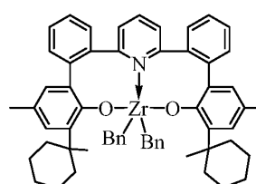
Complex 32
