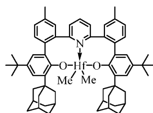
Complex 9
