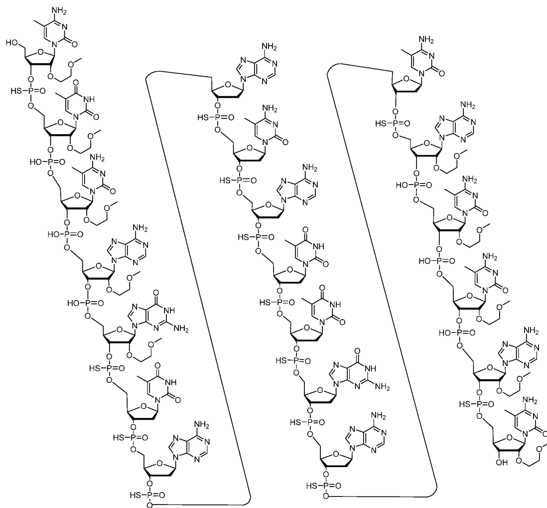
Structure 1. ISIS 443139
