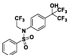
Structure of T0901317
