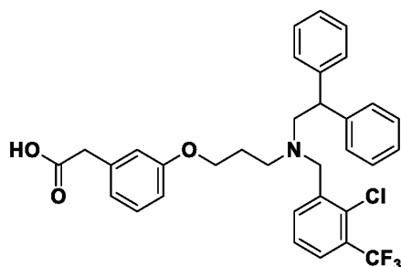
Structure of GW3965
