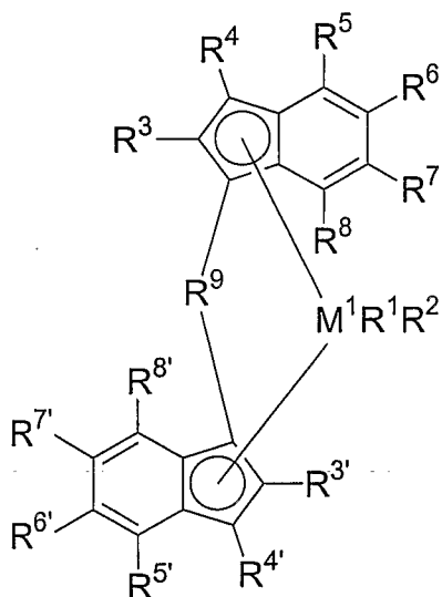
rac/pseudoracemic isomer
