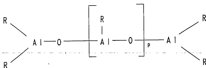
(Formula 4)
