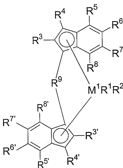
(Formula 1d)
