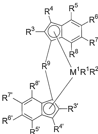
(Formula 1b)
