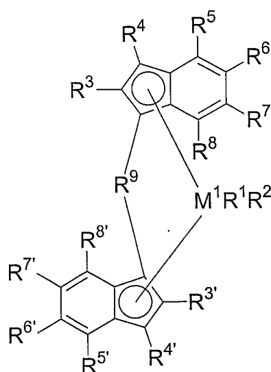
(Formula 1c)
