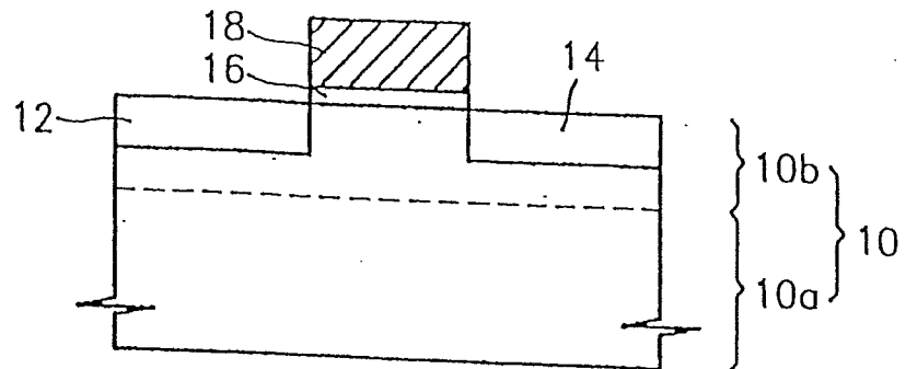
FIG. 1 (PRIOR ART)
