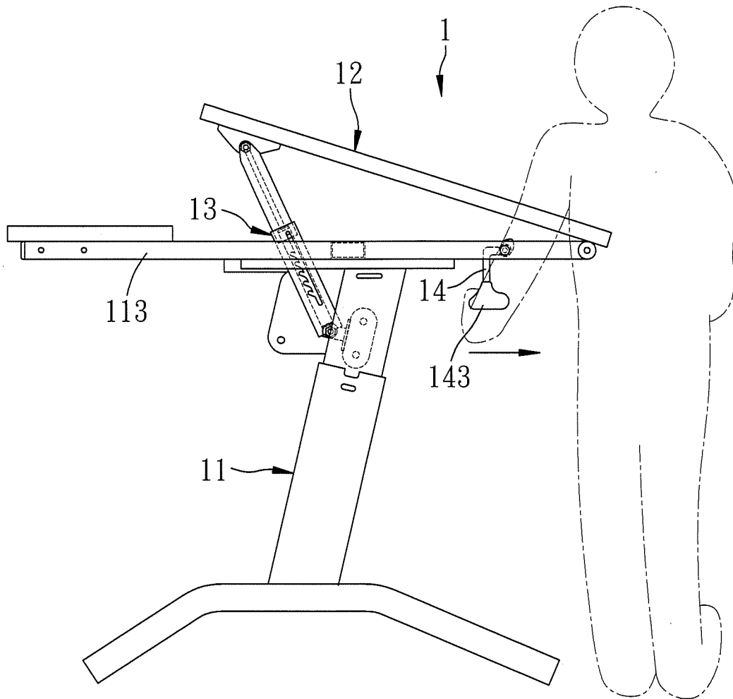
FIG. 4 PRIOR ART
