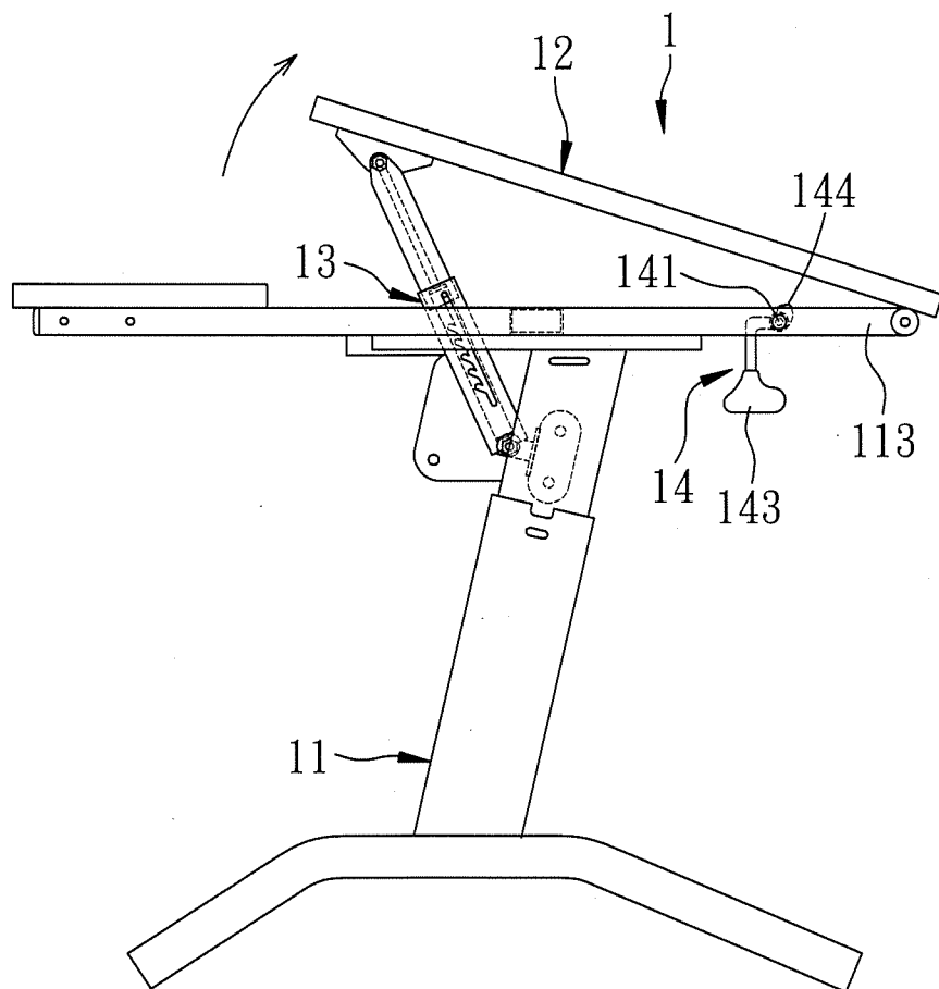
FIG. 1 PRIOR ART
