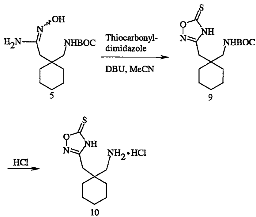
Scheme 5b
