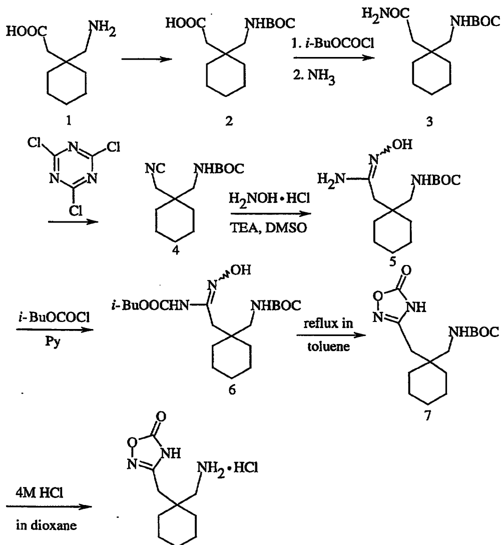
Scheme 5a
