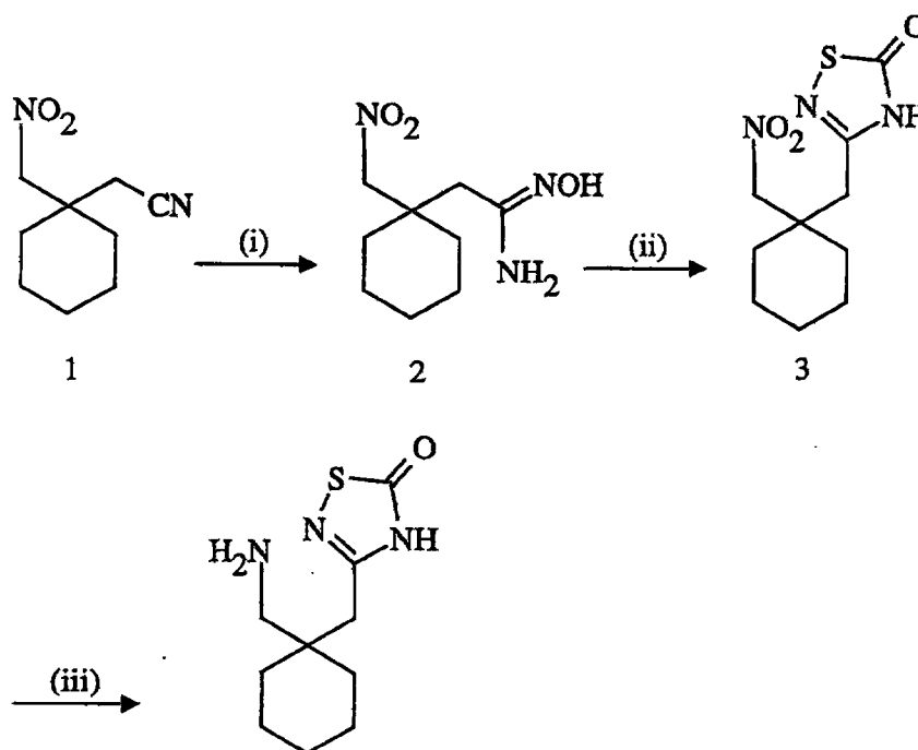
Scheme 7
