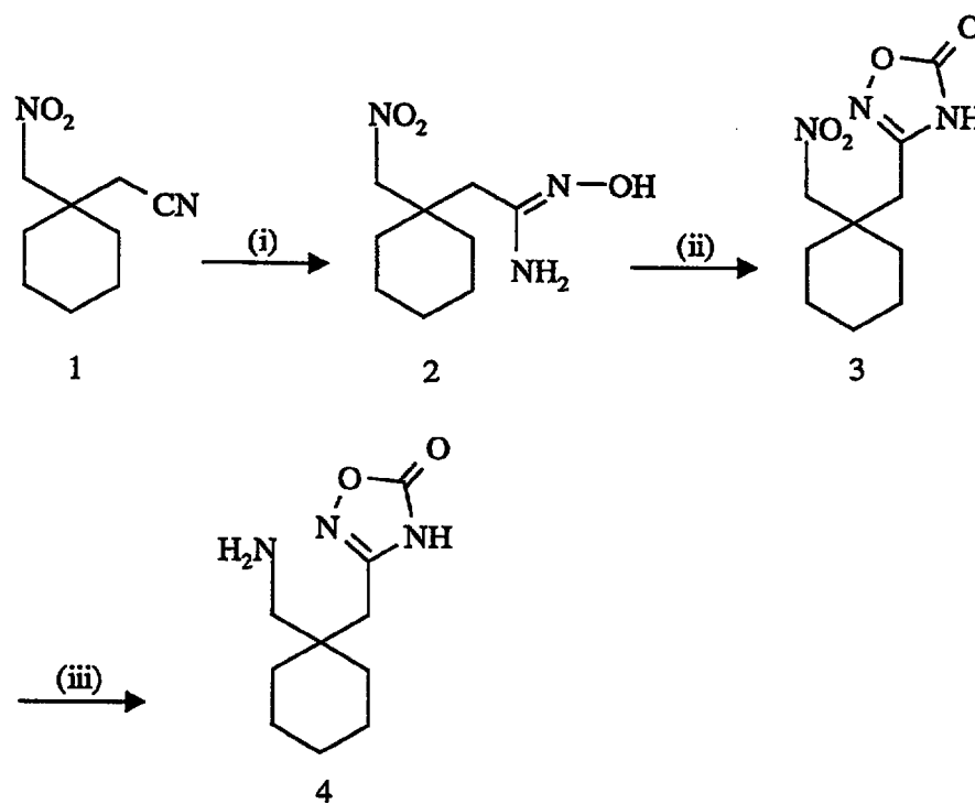
Scheme 4
