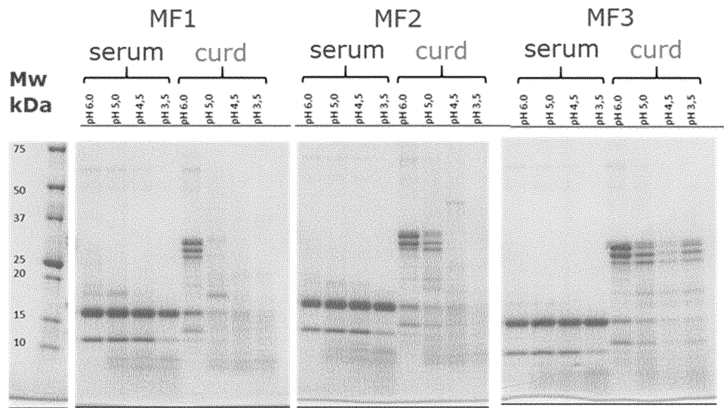
Figure 4 SDS-PAGE electrophoretograms of the model formulations
