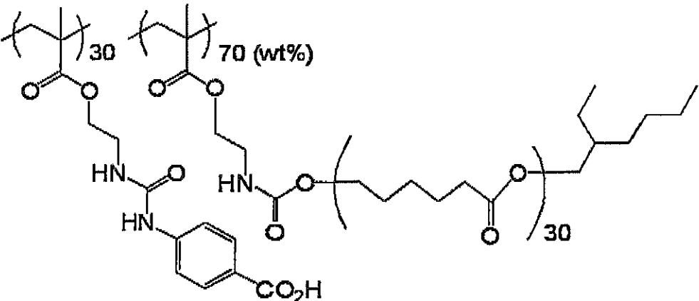
Exemplary Compound 40
