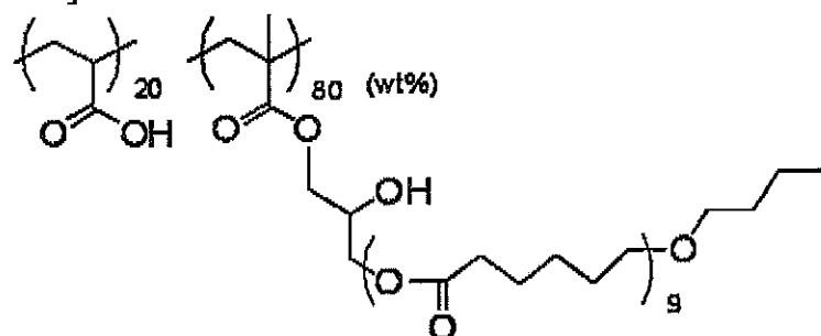
Exemplary Compound 32
