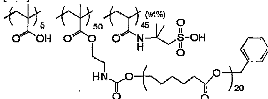
Exemplary Compound 24
