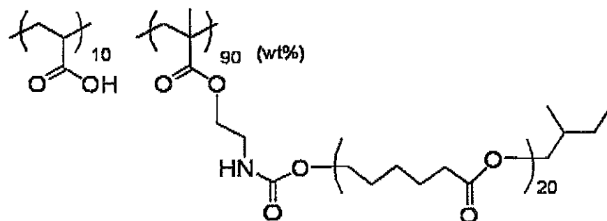
Exemplary Compound 19
