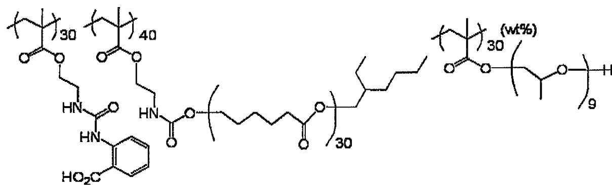
Exemplary Compound 49
