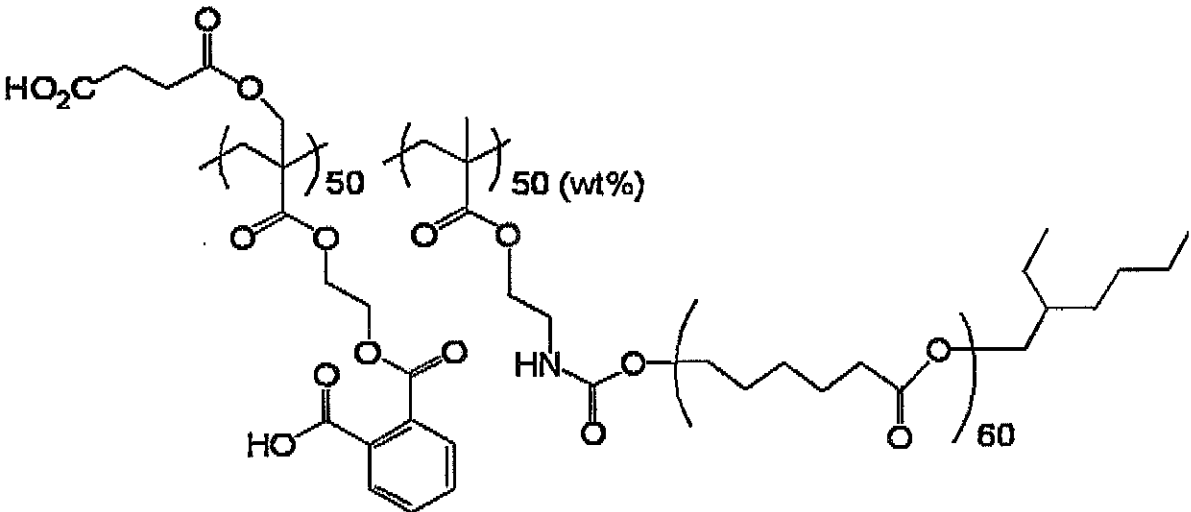
Exemplary Compound 41
