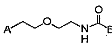
(Y-12)
