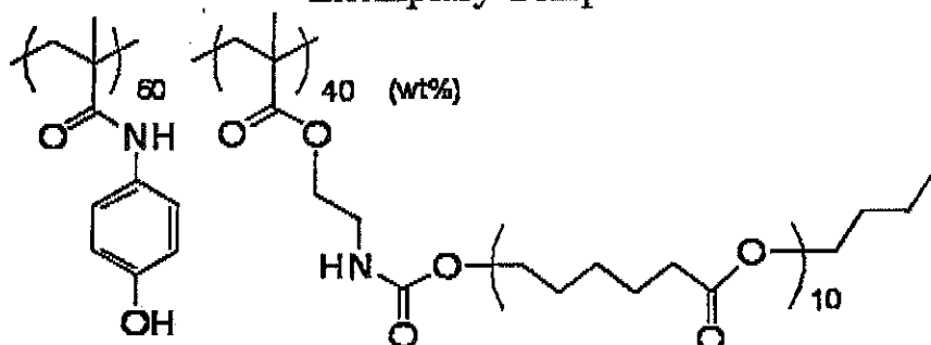
Exemplary Compound 25
