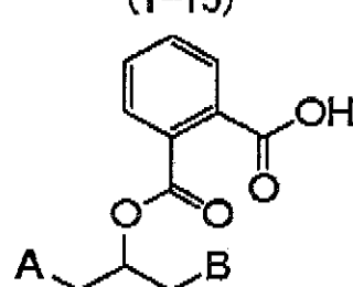
(Y-18)
