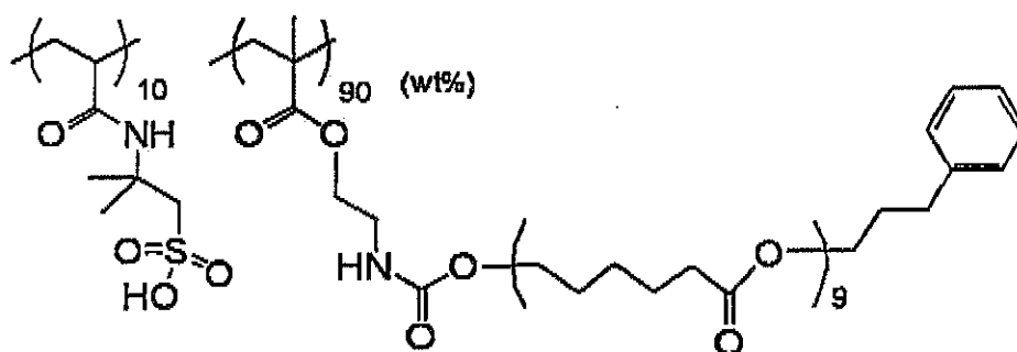
Exemplary Compound 17
