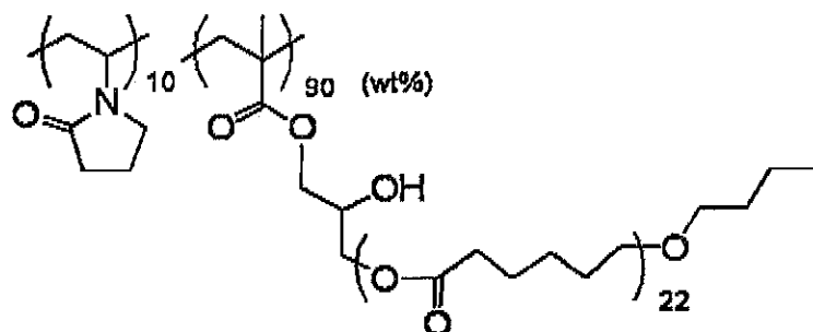
Exemplary Compound 33
