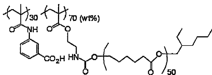
Exemplary Compound 44
