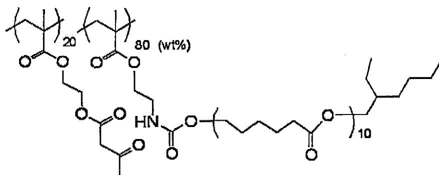
Exemplary Compound 30
