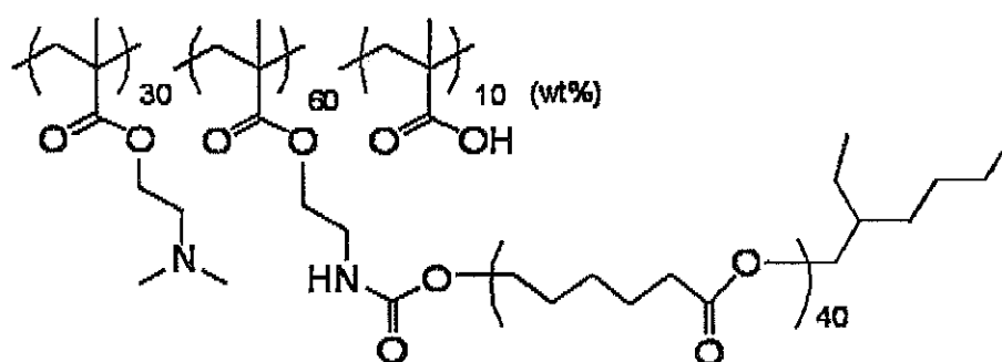
Exemplary Compound 27
