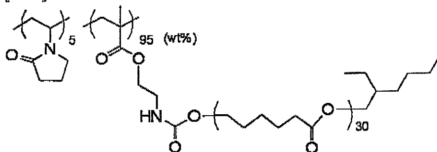
Exemplary Compound 28
