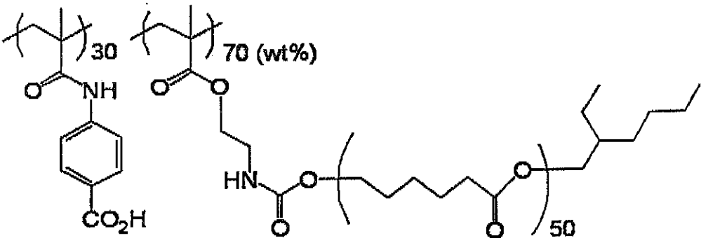
Exemplary Compound 42
