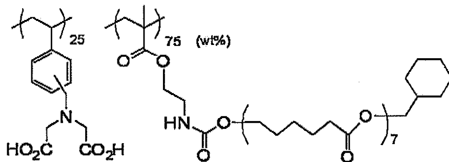
Exemplary Compound 18
