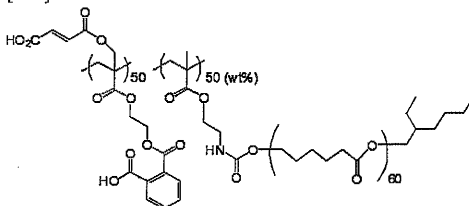
Exemplary Compound 43
