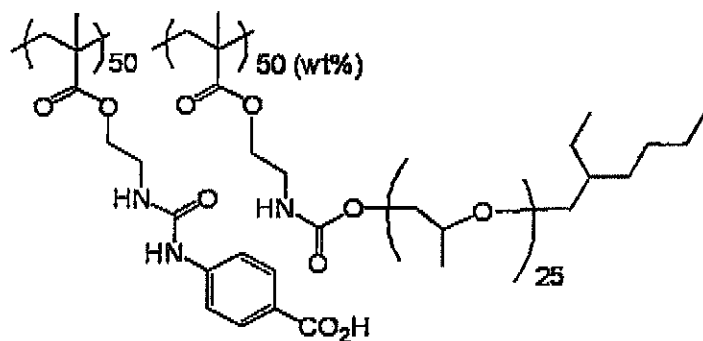
Exemplary Compound 45
