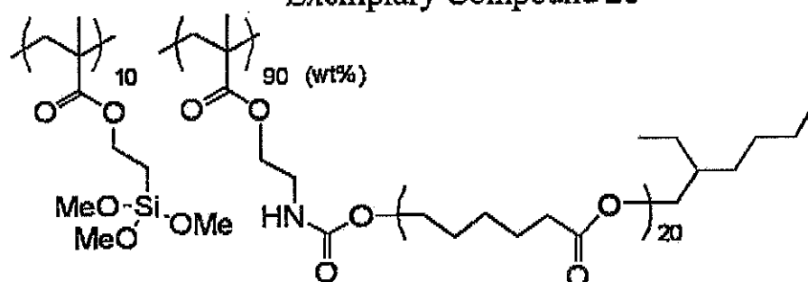
Exemplary Compound 29
