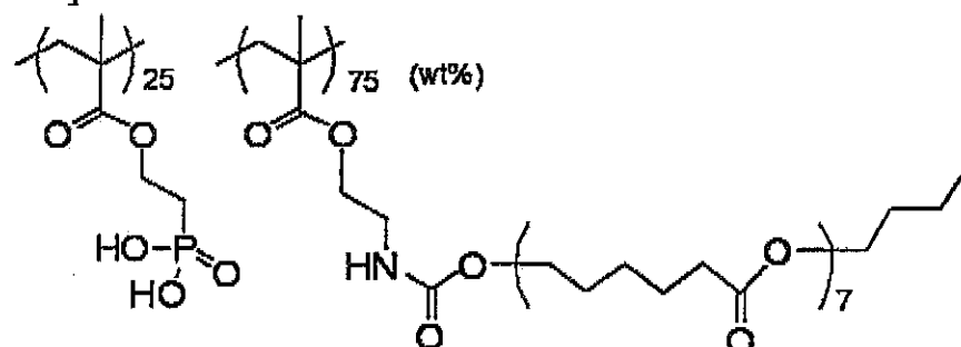
Exemplary Compound 16
