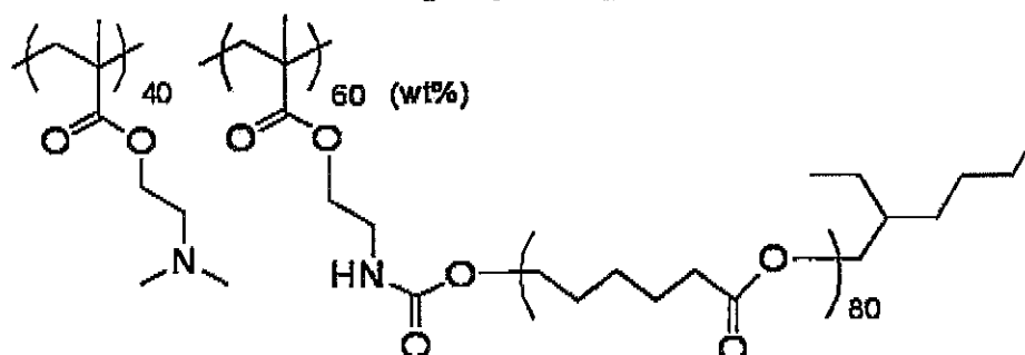
Exemplary Compound 26
