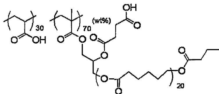
Exemplary Compound 34
