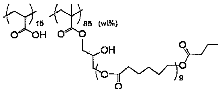
Exemplary Compound 31
