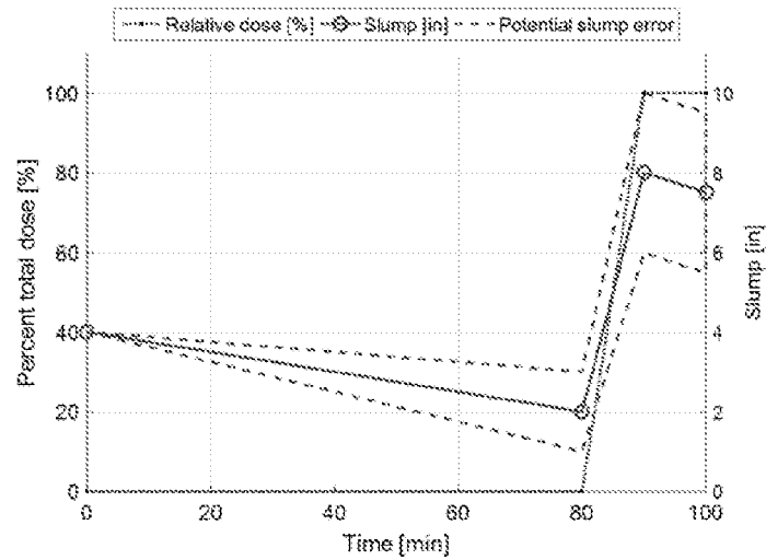
FIG. 3 (PRIOR ART)
