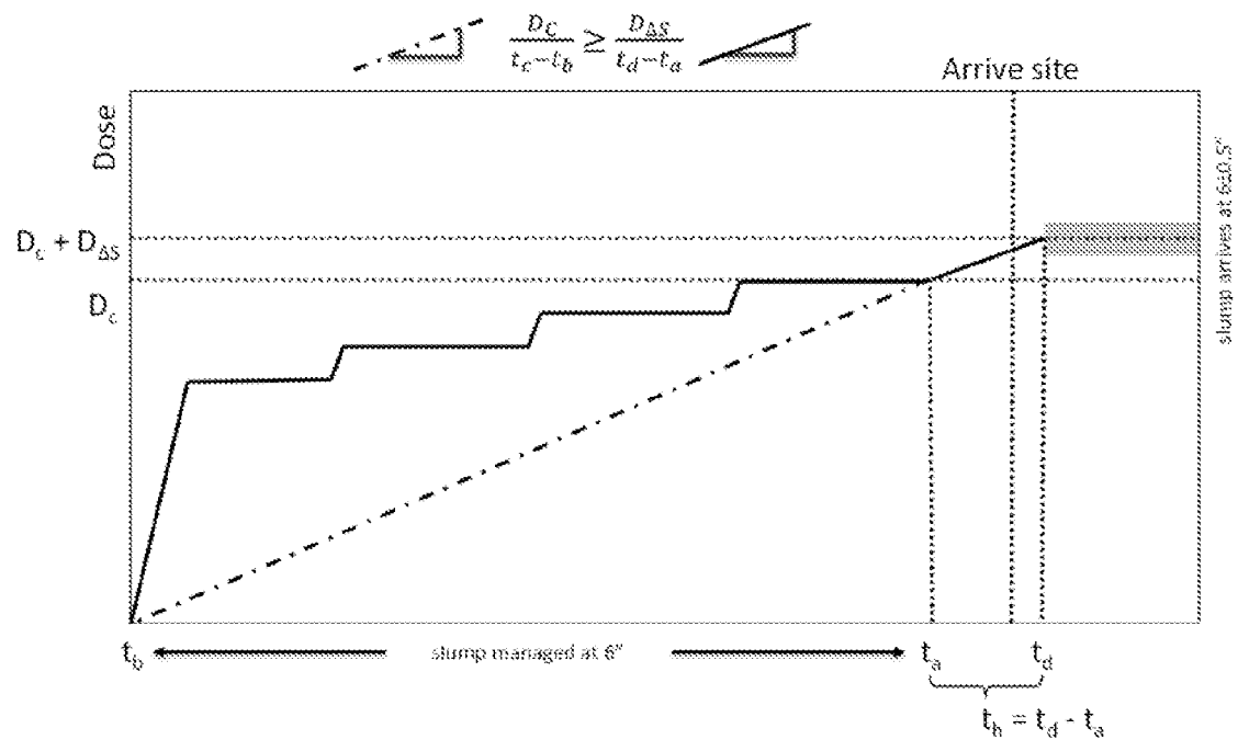
Fig. 7 (PRIOR ART)
