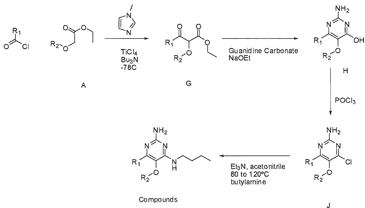
5 Scheme 4
