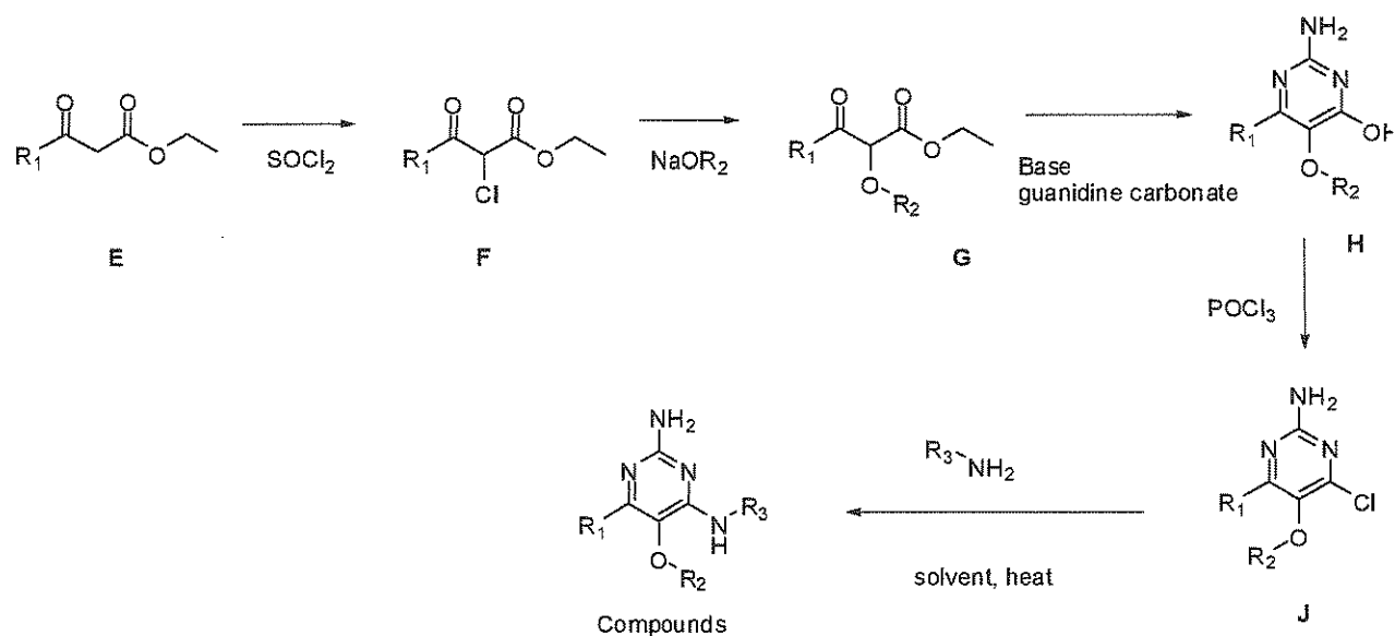
Scheme 3
