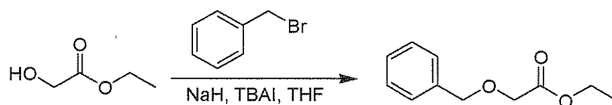
5 Scheme 2b
