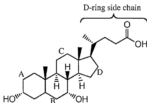
Chenodeoxycholic acid
