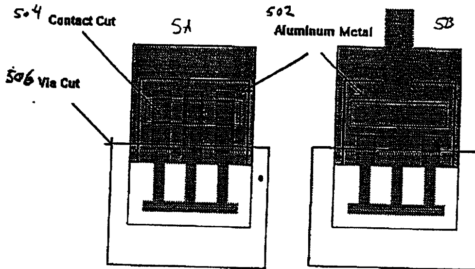
Fig 5 Metallization to sensor
