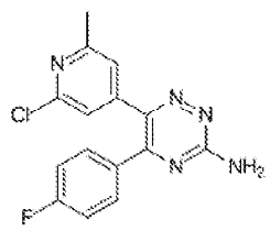
AZD4635
