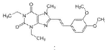
Istradefylline (KW-6002)
