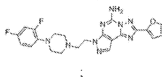
SCH-412,348
