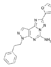
ST-1535
