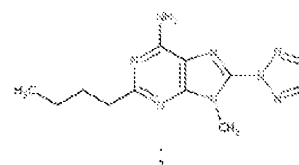
ST-1535
