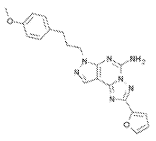
SCH-442,416
