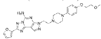
Preladenant (SCH-420,814)
