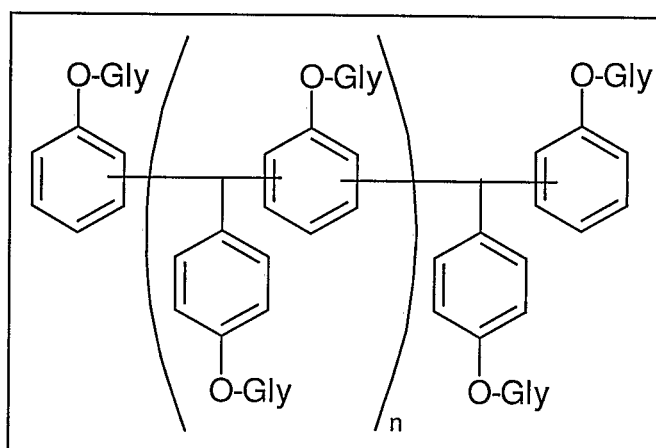
Fig.2 tris phenol type epoxy
