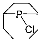
Asym-PhobPCI
