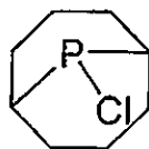
Sym-PhobPCI
