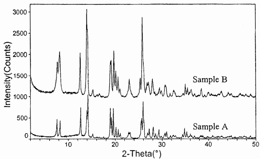
Figure 3. Comparison of Samples A &amp; B
