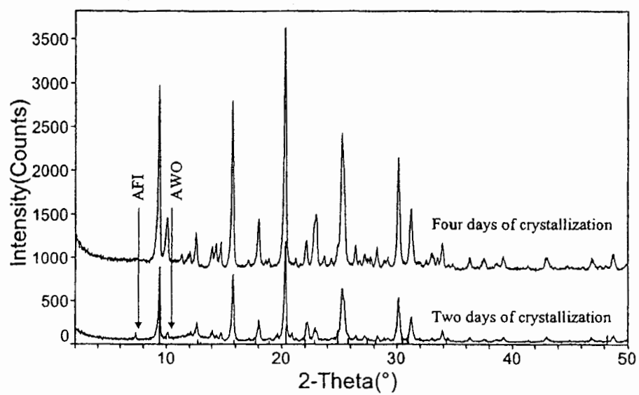
Figure 8. XRD Patterns of Example 8
