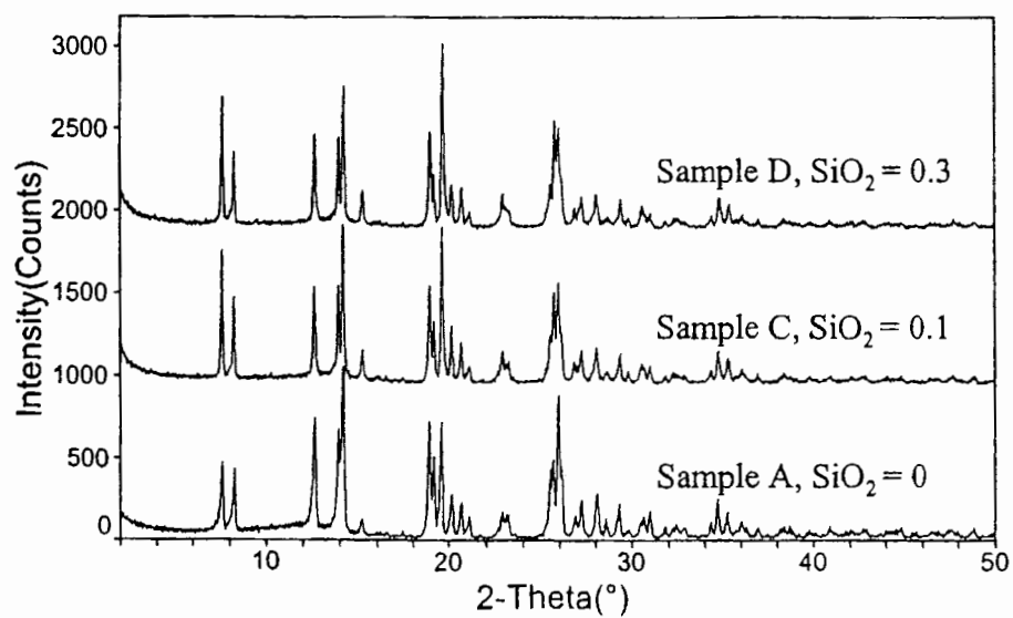
Figure 5. XRDs of Samples A, C, &amp; D
