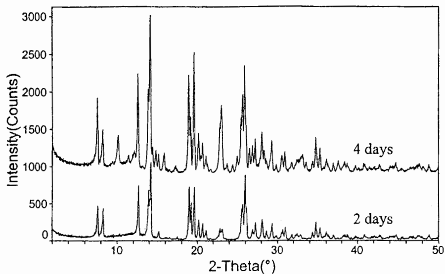
Figure 2. XRD's of Example 1 Products
