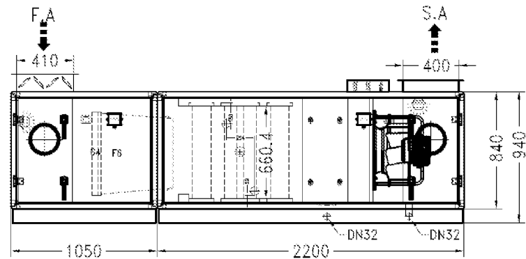
FIGURE 7: Side view of the ICON PCC with an approximate dimension
