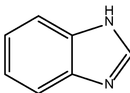
Figure 1: Benzimidazole
