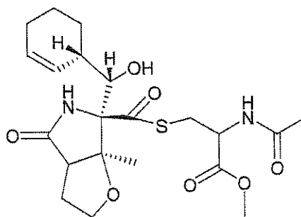
Formula VI-1C
