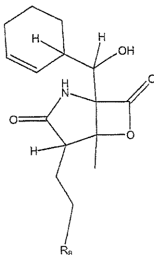
Formula II-15
