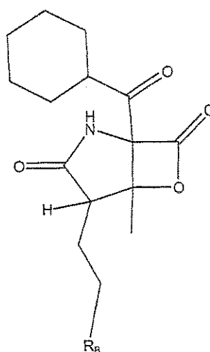
Formula II-8
