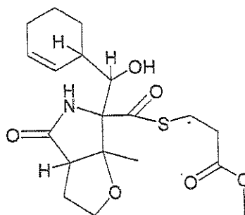
Formula VI-1A
