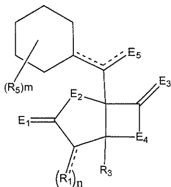
Formula IV
