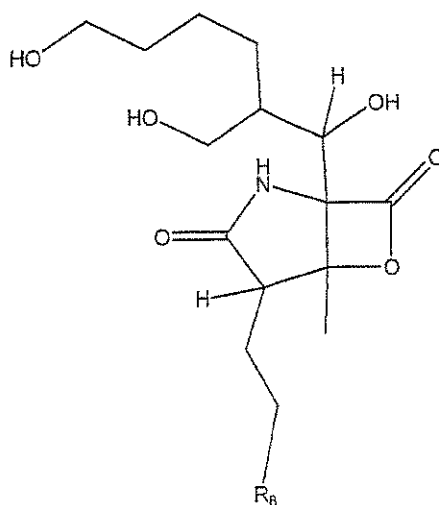
Formula II-6
