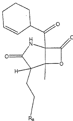
Formula II-13
