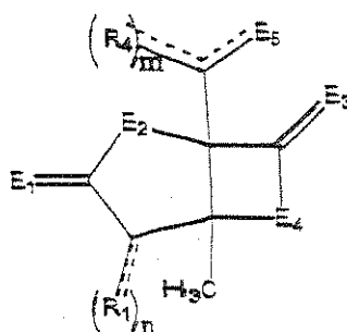
Formula III
