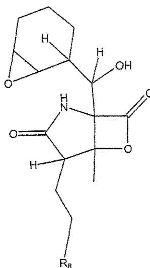
Formula II-5
