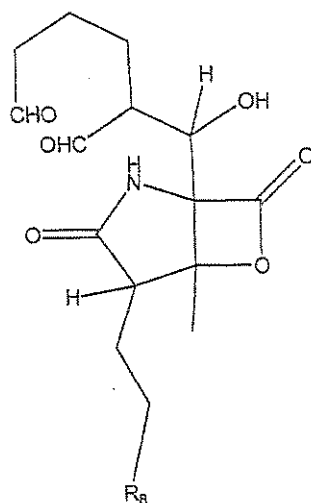
Formula II-7
