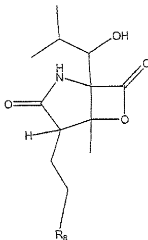
Formula II-10
