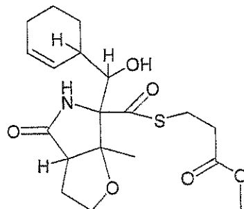
Formula VI-1A
