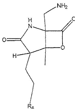
Formula I-5
