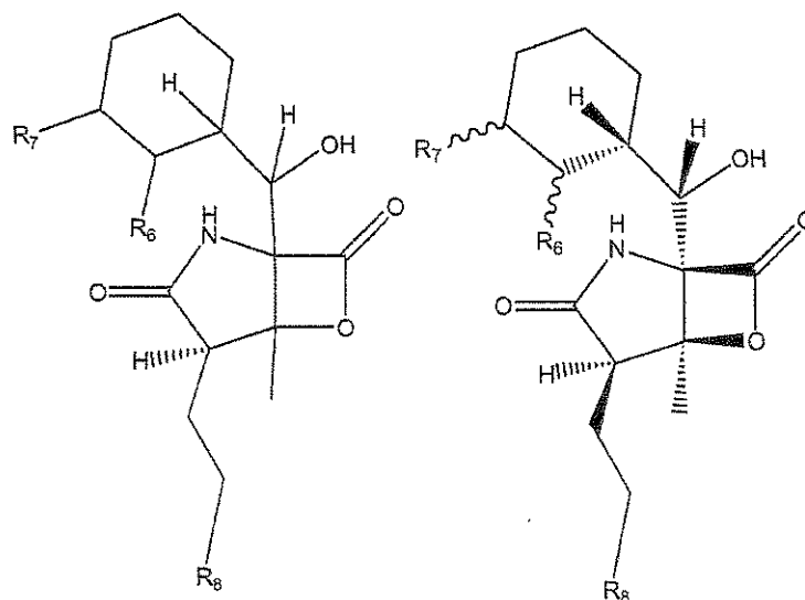
Formula IV-1
