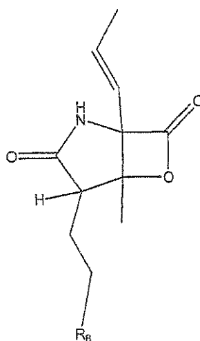
Formula I-3
