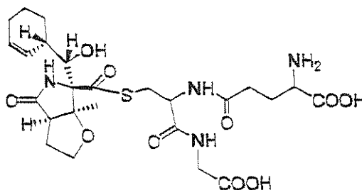
Formula VI-1B
