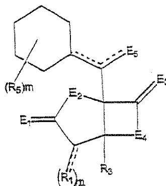
Formula IV
