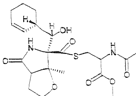
Formula VI-1C
