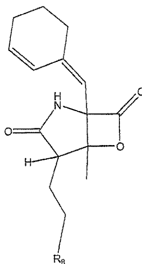
Formula I-6
