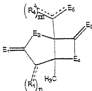
Formula III
