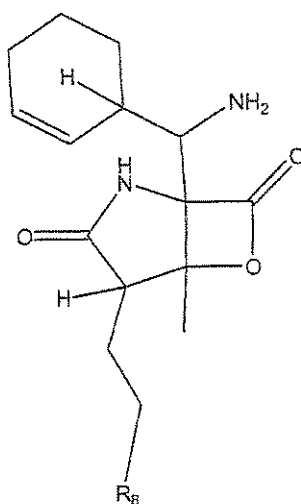
Formula II-11
