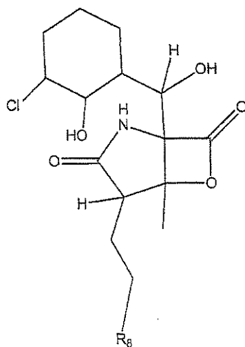
Formula IV-3
