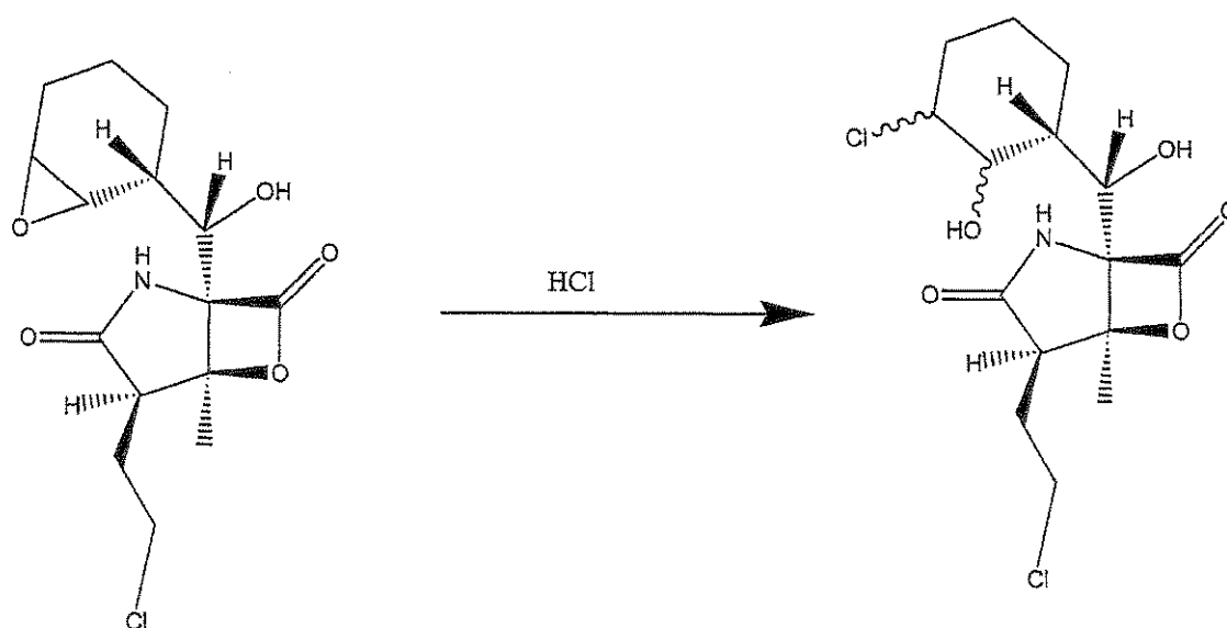
Formula II-5
