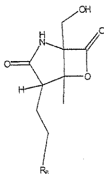
Formula I-2
