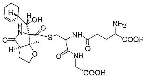
Formula VI-1B
