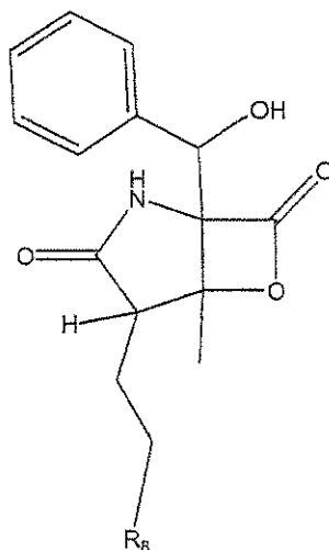
Formula II-14
